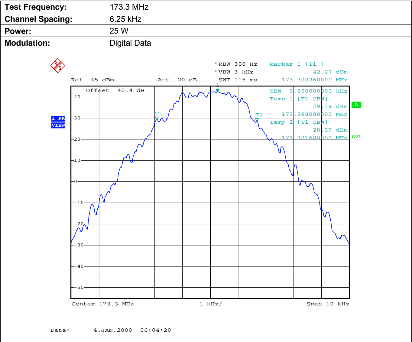
Plot 5.7.4.1.6. Occupied Bandwidth
