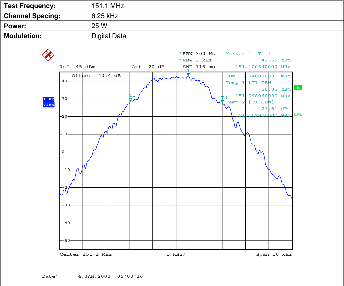
Plot 5.7.4.1.5. Occupied Bandwidth
