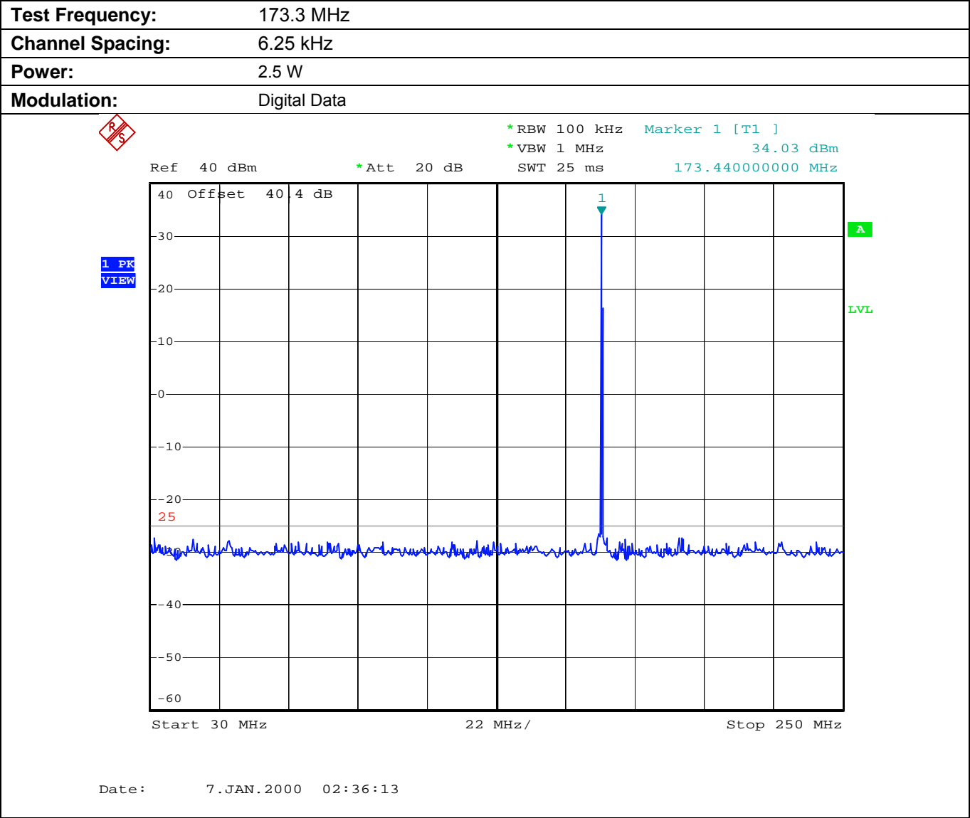
Plot 5.8.4.3.3. Conducted Transmitter Spurious Emissions for 173.3 MHz, Low Power, 30 MHz - 250 MHz
