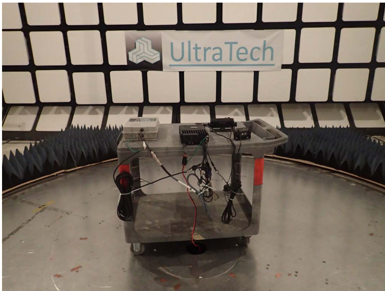
Radiated Emission at 3m
