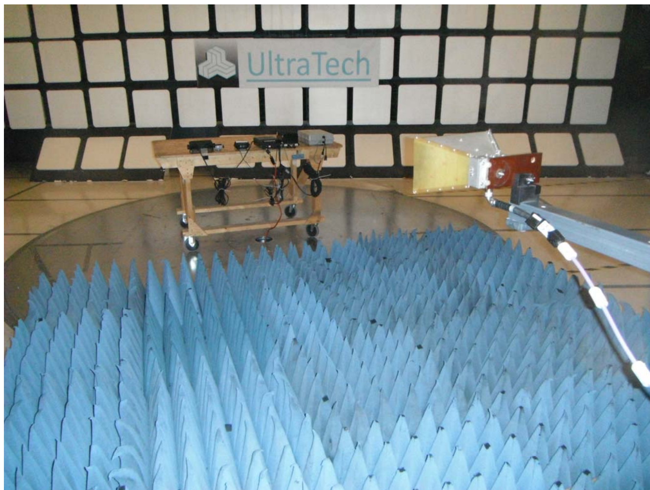
Radiated Emission at 3m, Above 1GHz
