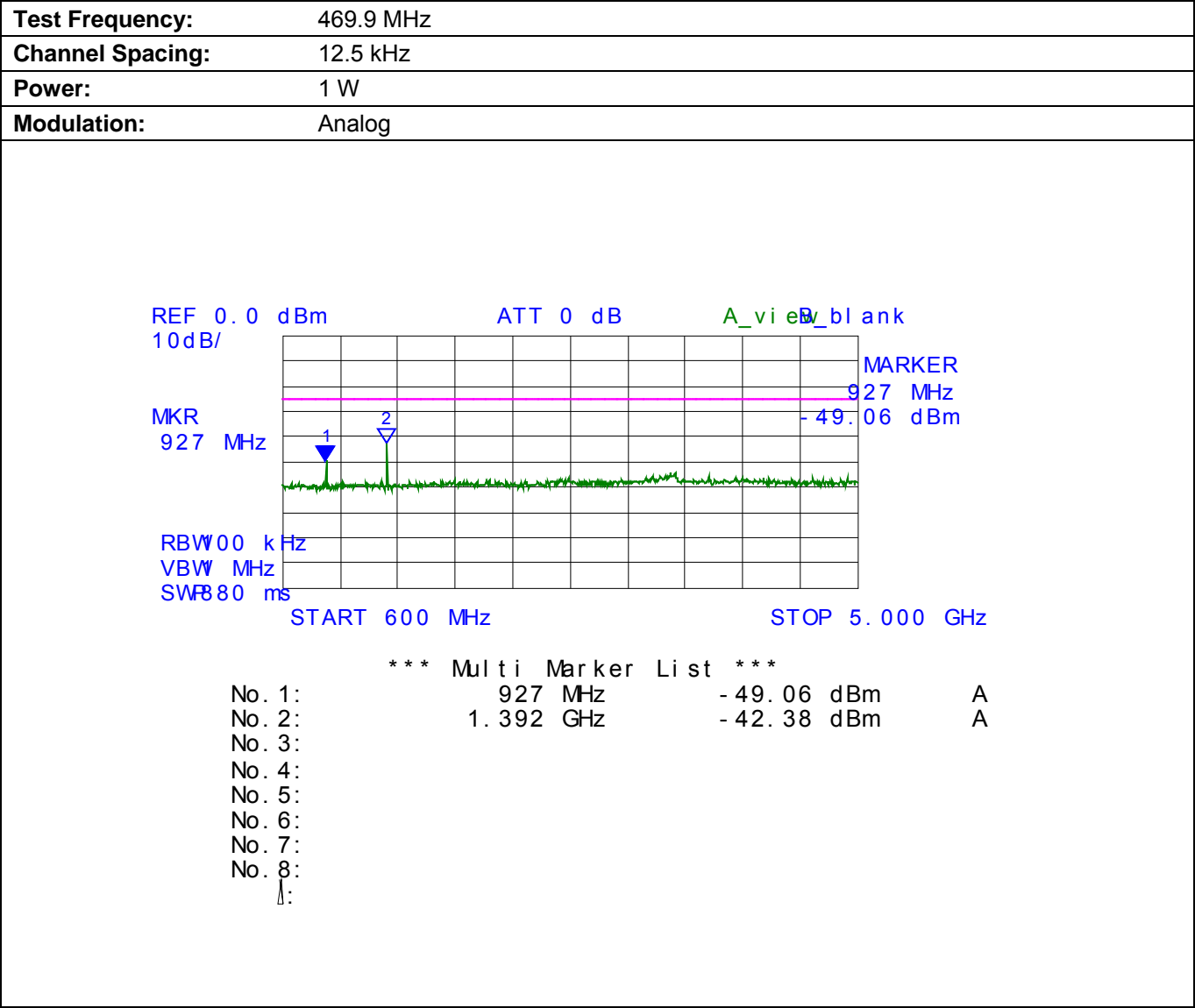
Plot 5.9.4.3.4. Conducted Transmitter Spurious Emissions for 469.9 MHz, Low Power, 600 MHz - 5 GHz
