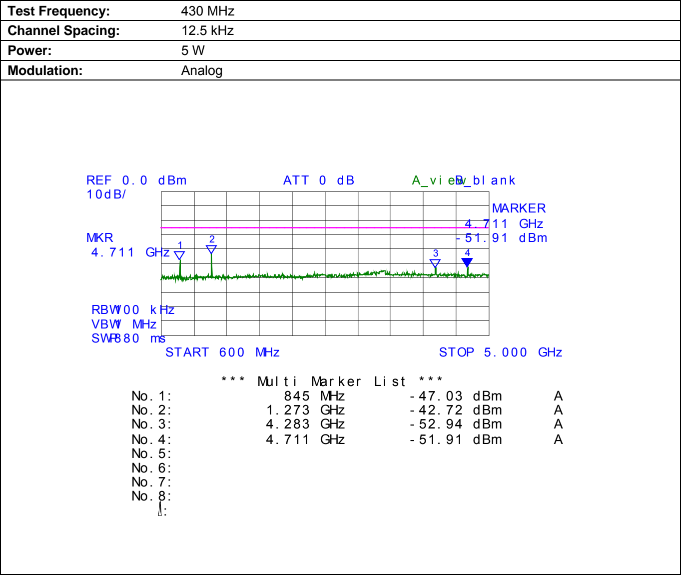
Plot 5.9.4.2.2. Conducted Transmitter Spurious Emissions for 430 MHz, High Power, 600 MHz - 5 GHz
