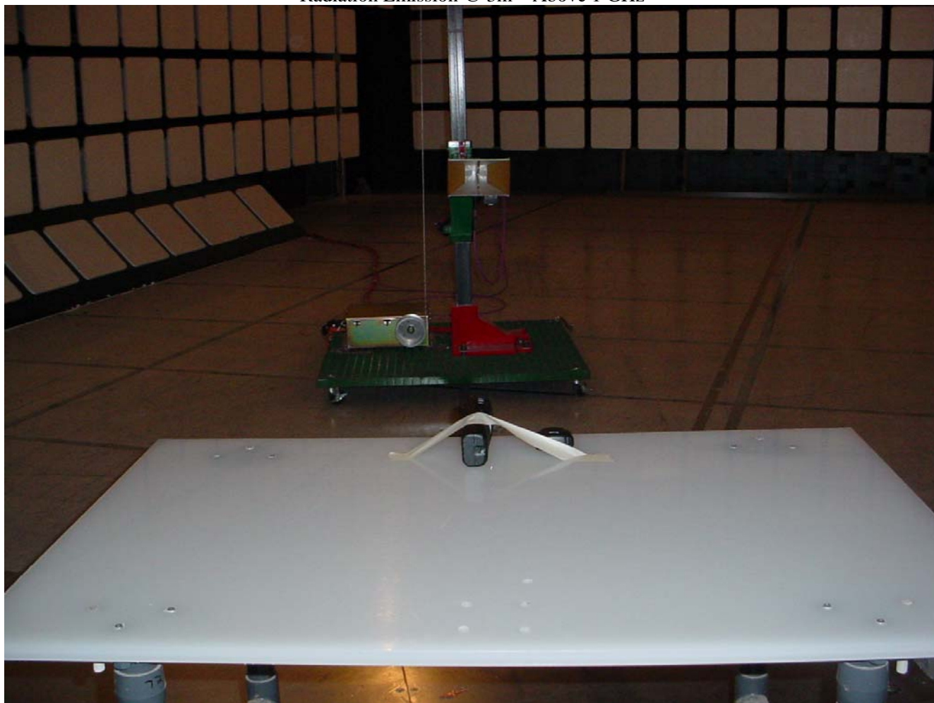
Radiation Emission @ 3m – Above 1 GHz
