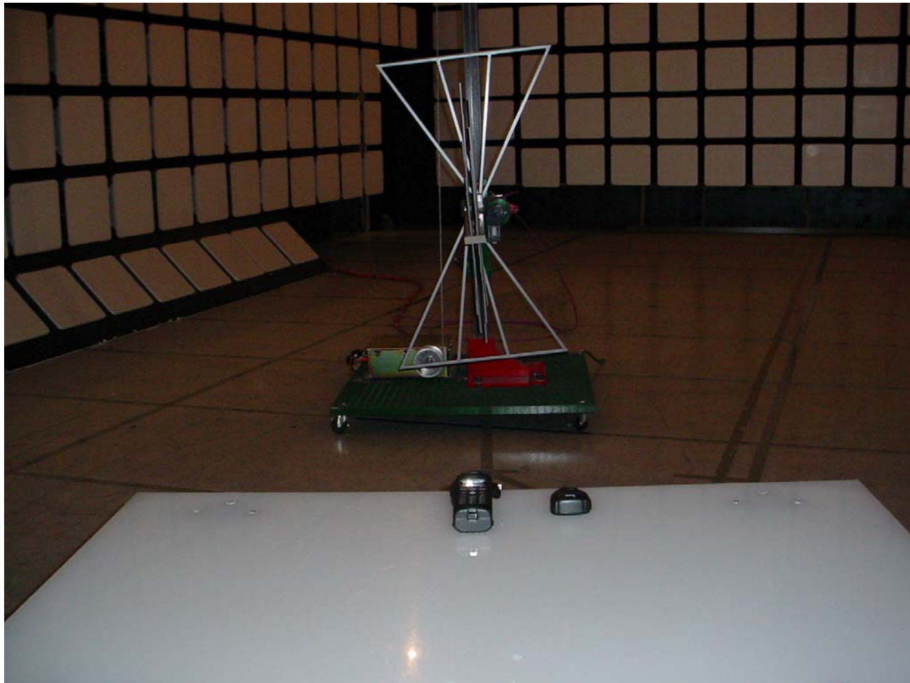
Radiation Emission @ 3m – Below 1 GHz
