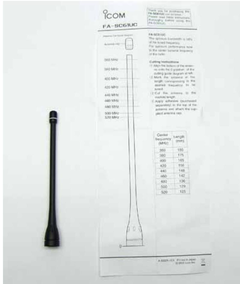
< FA-SC61UC cut antenna with the length of 129mm >
