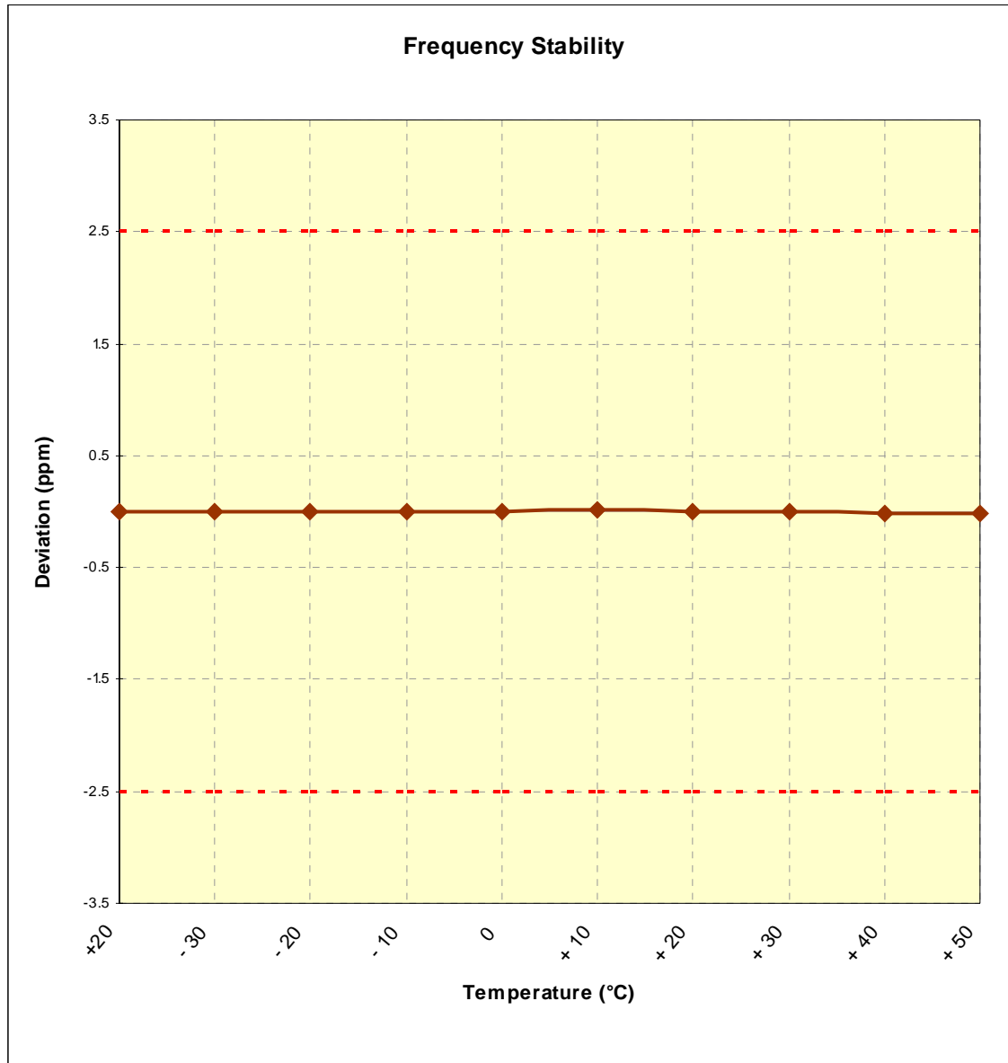
Figure 6-2. Frequency Stability Graph (PCS CDMA Mode – Ch. 600)
