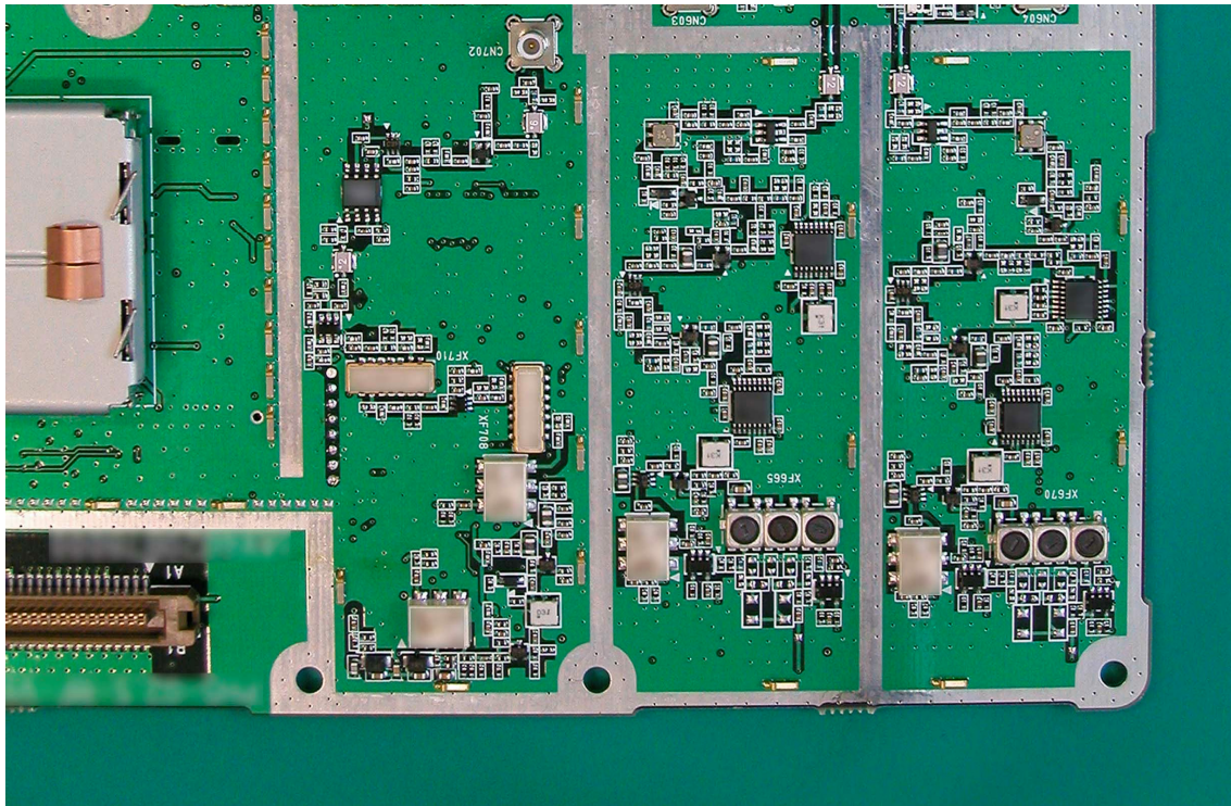
21-4 *RFMB board –front view (Part 4)
