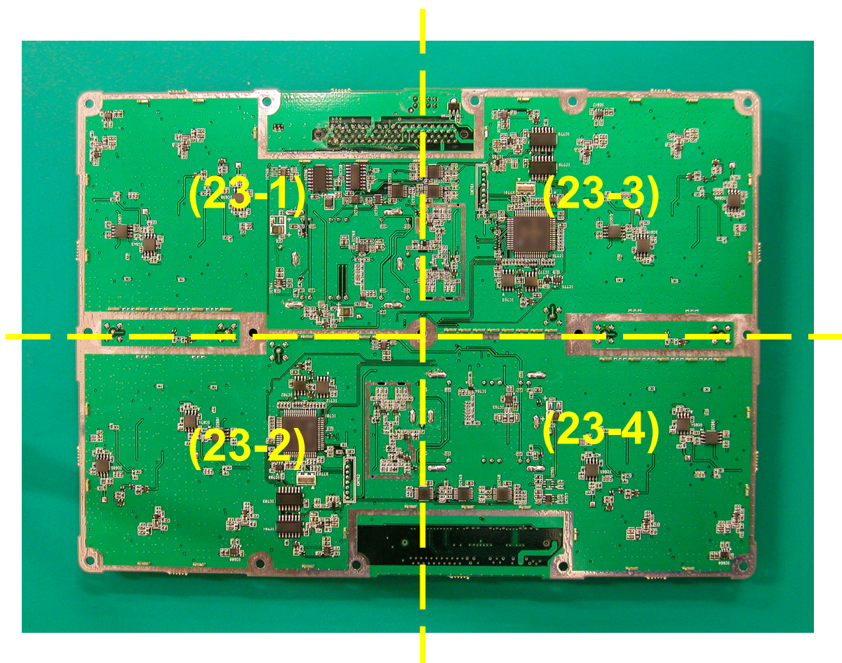
23 RFMB board (back view)
