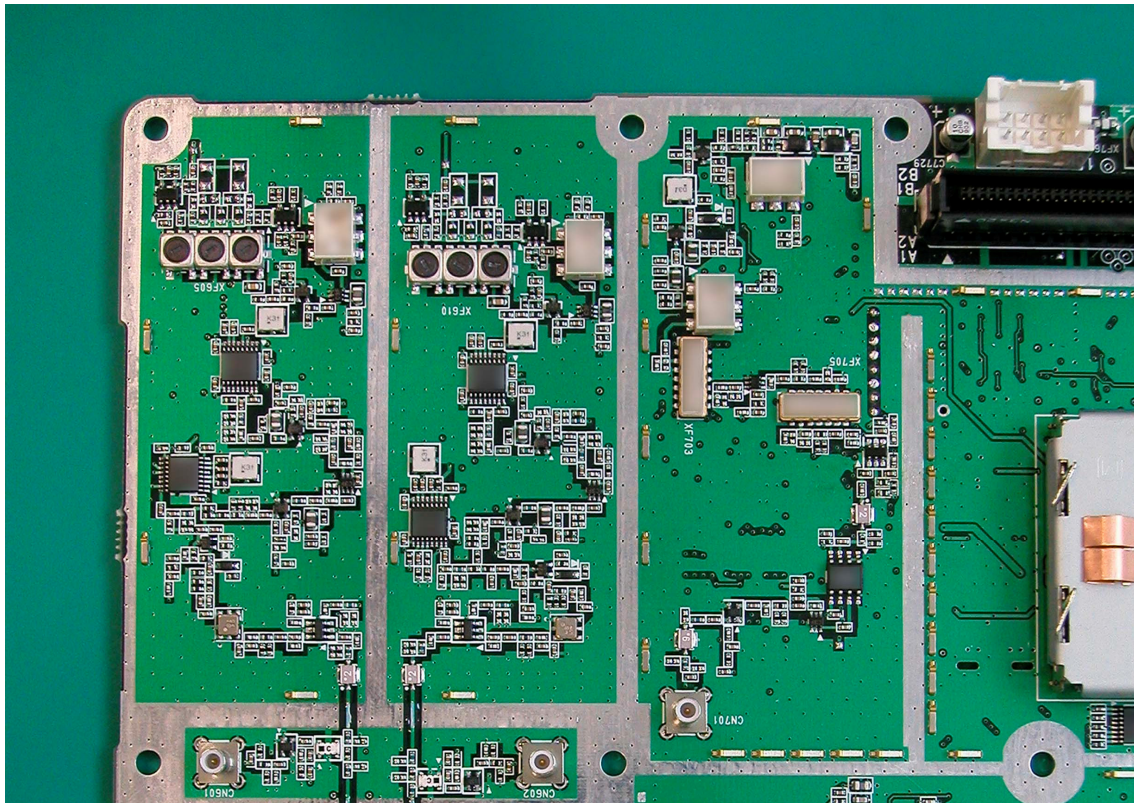
21-1 *RFMB board –front view (Part 1)
