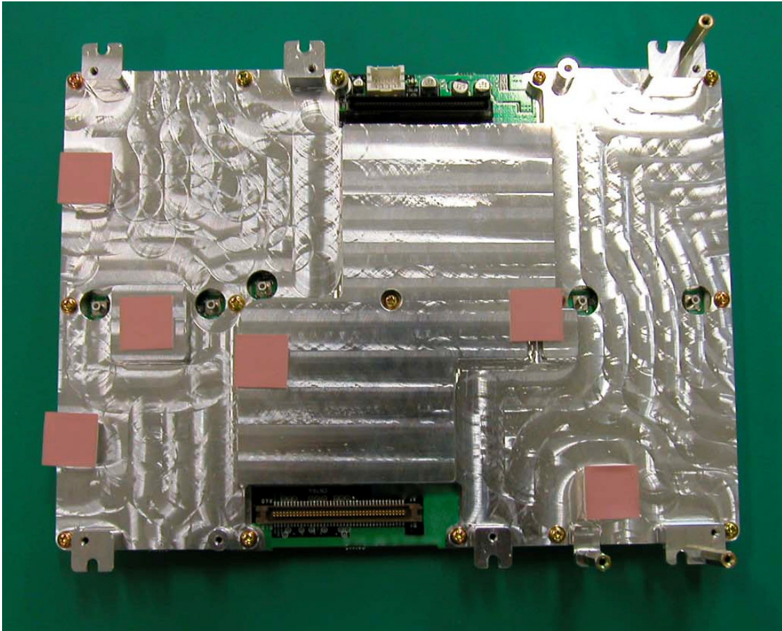
19 RFMB board (with sealed case, front view)
