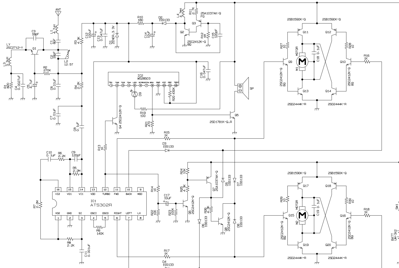
RECEIVER TY-W2283-1 27MHZ Drawing No. TAIYO KOGYO CO., LTD
