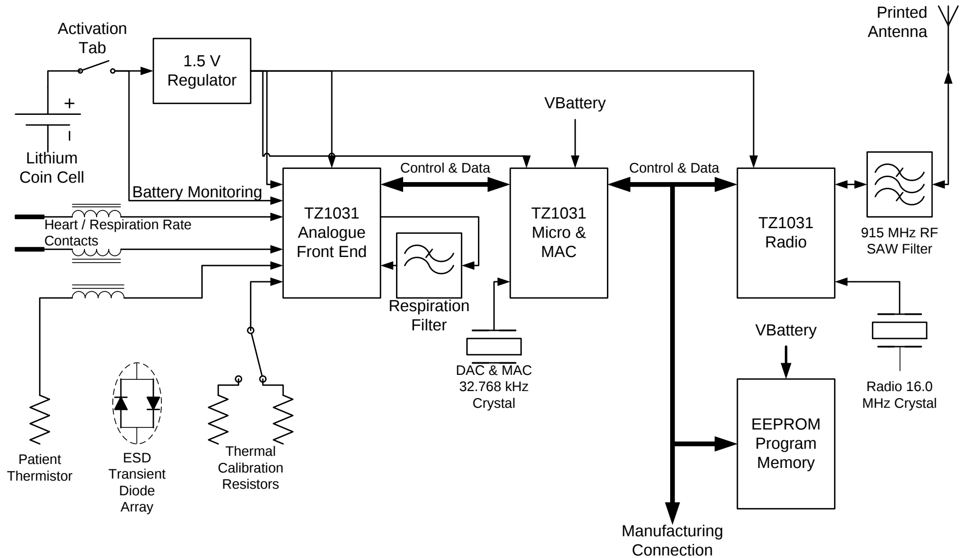
TZ202055 Patch Block Diagram
