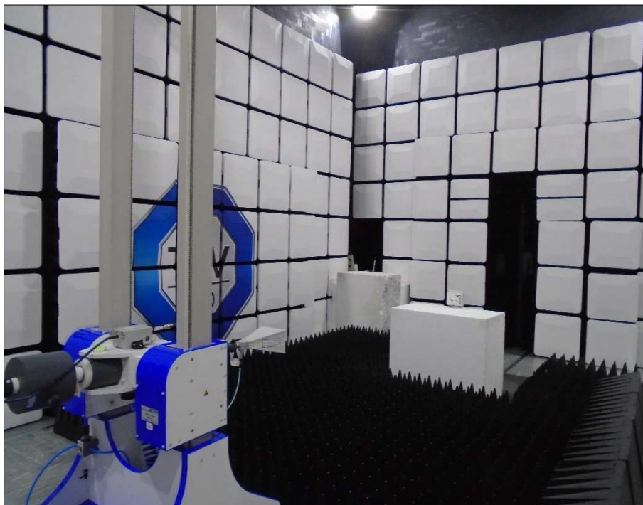
Figure 2 – Radiated Disturbance - 1 GHz to 5 GHz
