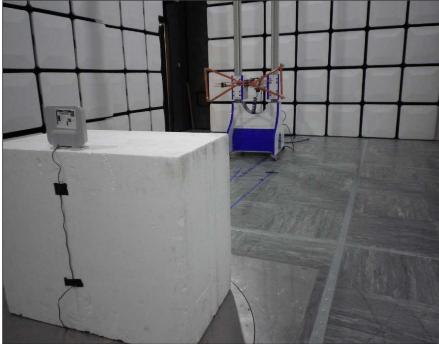
Figure 1 – Radiated Disturbance - 30 MHz to 1 GHz
