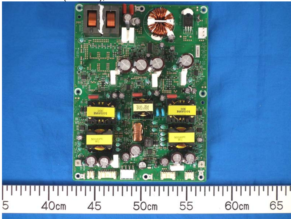
1.5 PWR Board (03P9679), Front side
