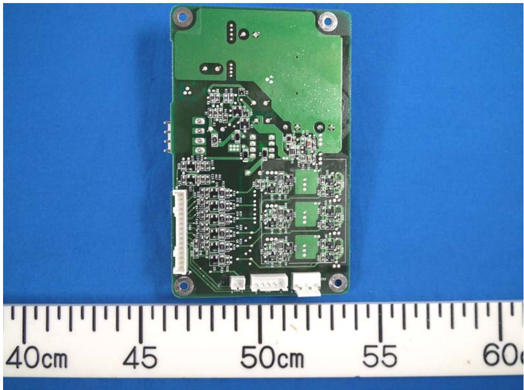
1.8 MTR-DRV Board (14DJ003 (MD-DJ-B48)), Rear side
