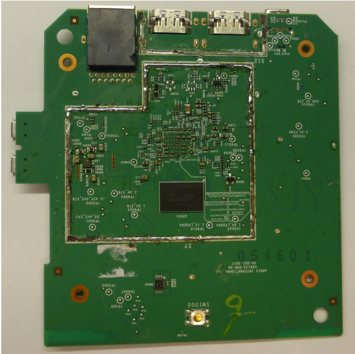
PCB Bottom (Shields Removed)
