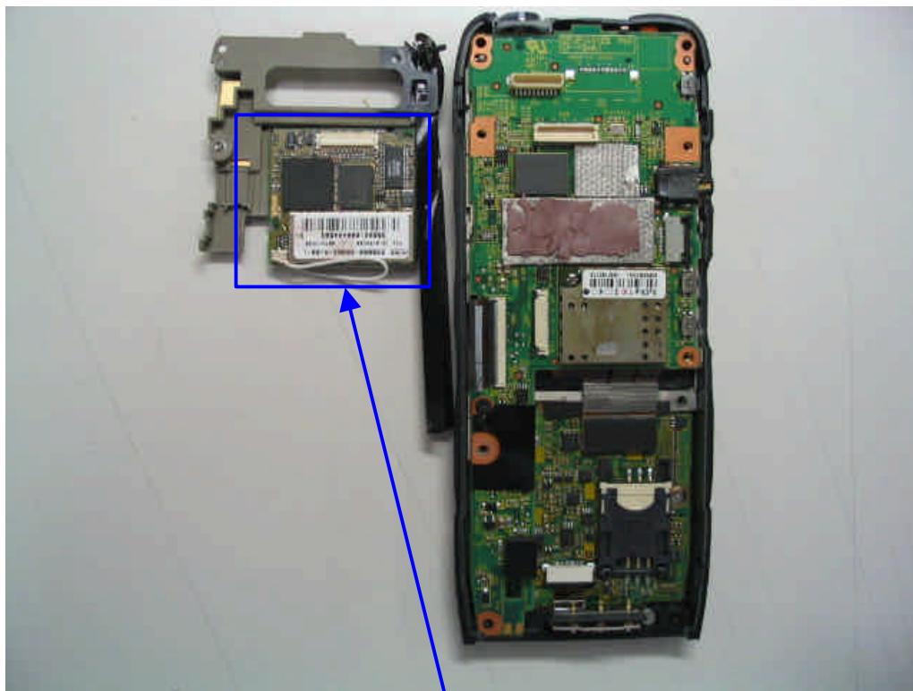
MC56 Module Position
