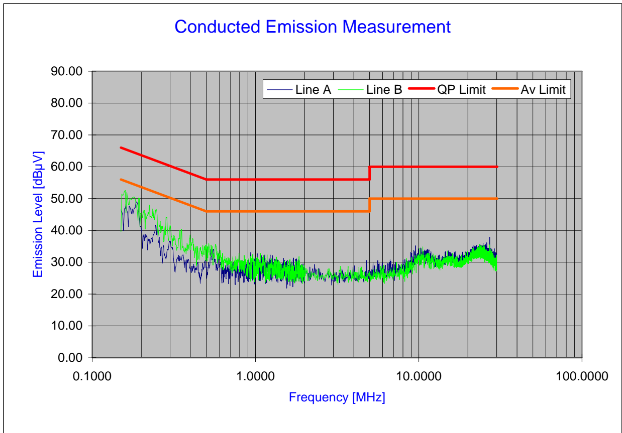
Plot 6-78. Line Conducted Plot with 802.11a
