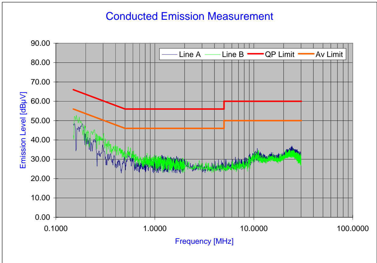
Plot 6-77. Line Conducted Plot with 802.11g
