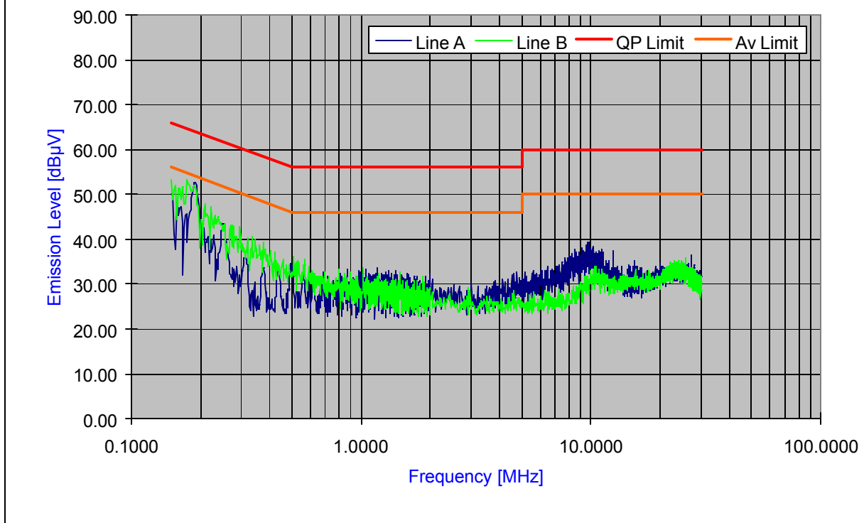
Plot 6-51. Line Conducted Plot with 802.11a (UNII Band III)
