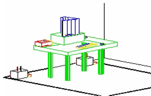
Figure 3-2. Line Conducted Emission Test Set-Up
