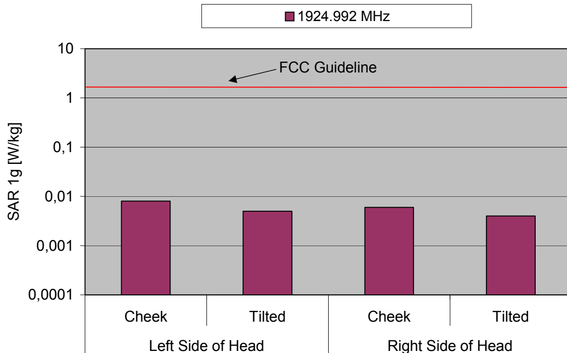
Fig. 8: The measured head phantom SAR values for the Panasonic KX-WT126 for the US DECT standard in comparison to the FCC exposure limit.
