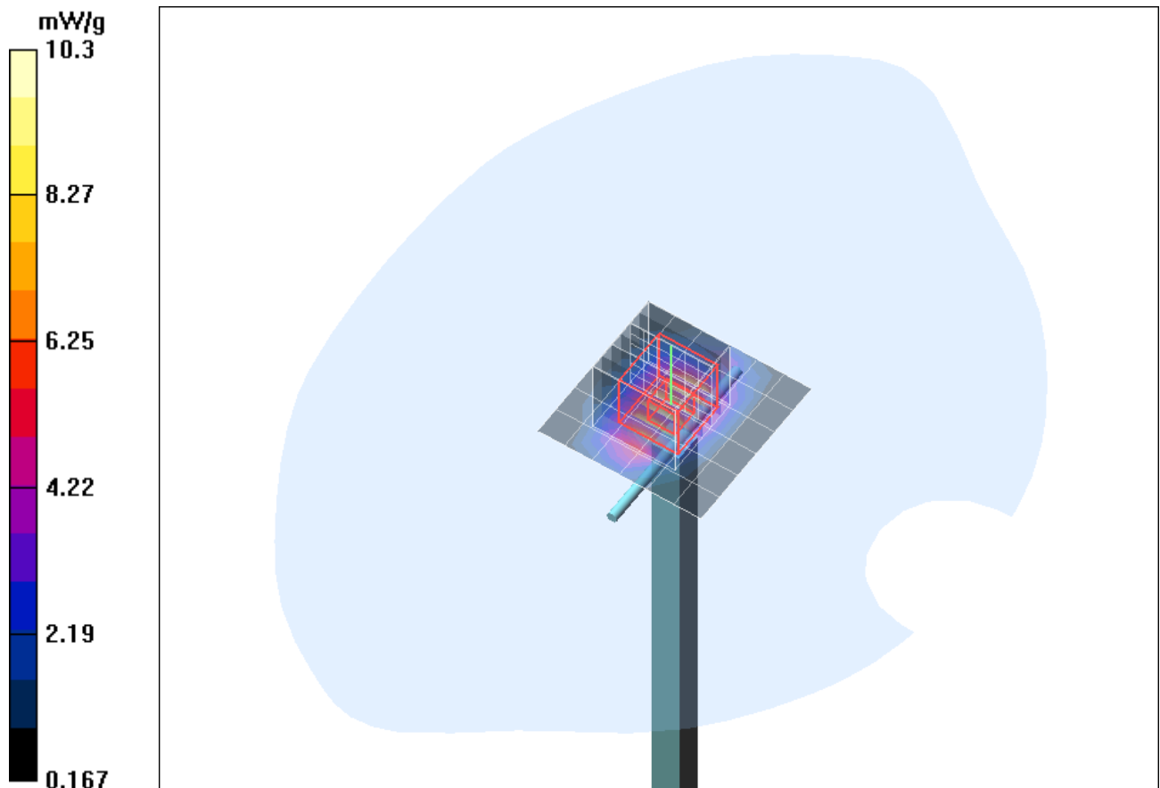
Fig. 11: Validation measurement 1900 MHz body (August 24, 2010), coarse grid. Ambient Temperature: 22.4° C, Liquid Temperature: 21.8° C.
