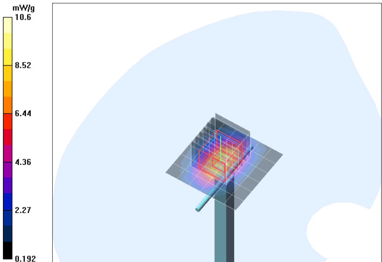
Fig. 10: Validation measurement 1900 MHz Head (August 25, 2010), coarse grid. Ambient Temperature: 22.1° C, Liquid Temperature: 21.7° C.
