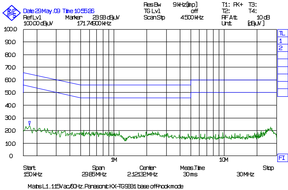
Off-Hook Mode, Phase L1
