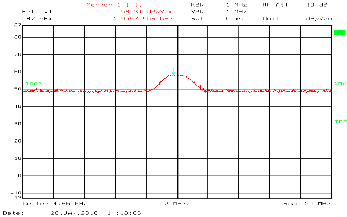
Radiated emissions, 2 nd harmonic, ch78
