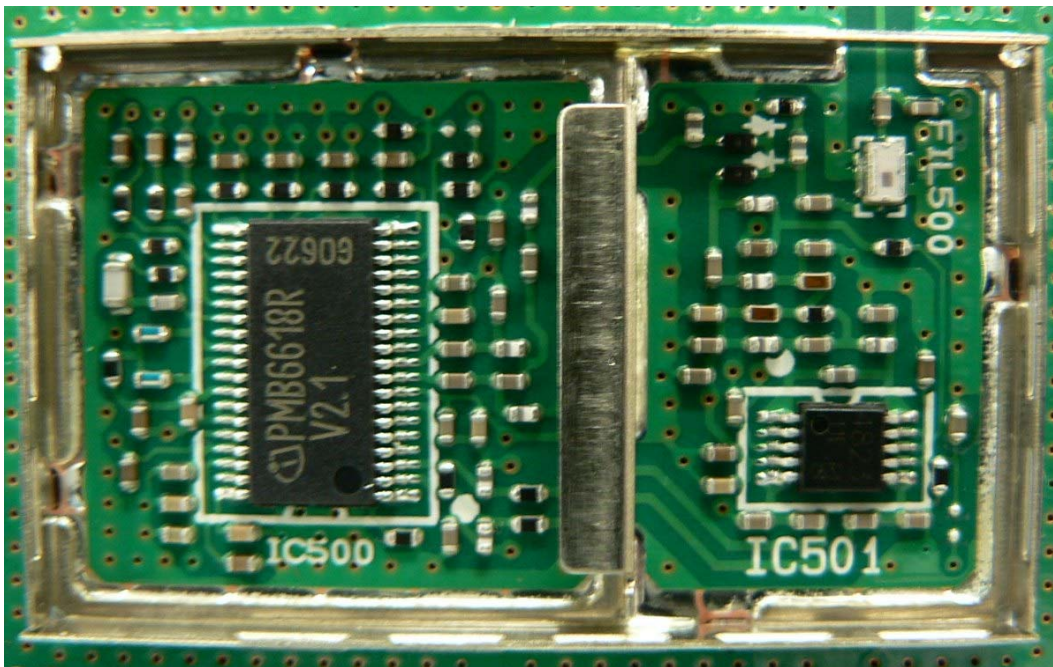
RF block of KX-TDA0152 and KX-T0151, View of under the shield case
