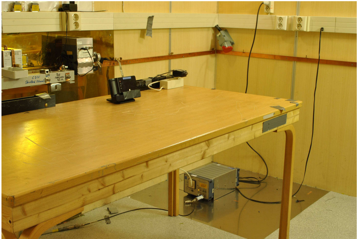
Power line Conducted Emissions Test, BT
