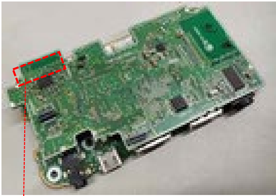
Antenna is placed on the top PCB(TNPA8056)
