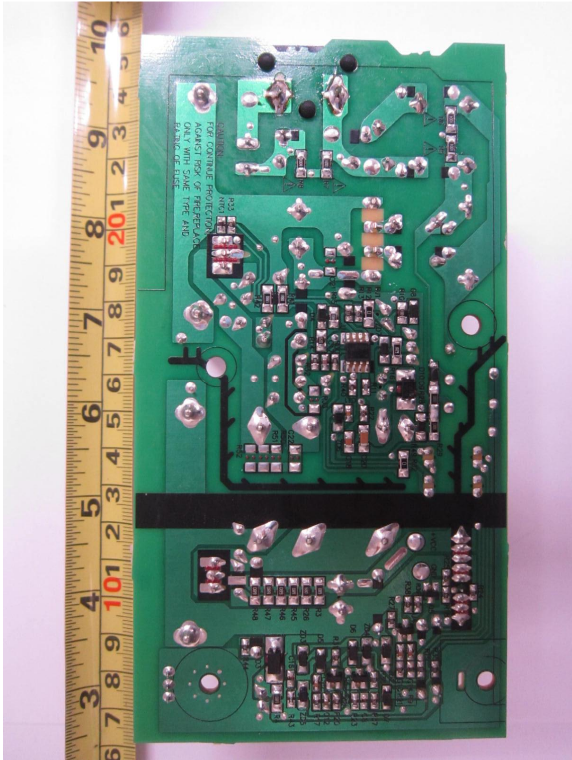
Power Supply Sub-Board PCB Trace Side
