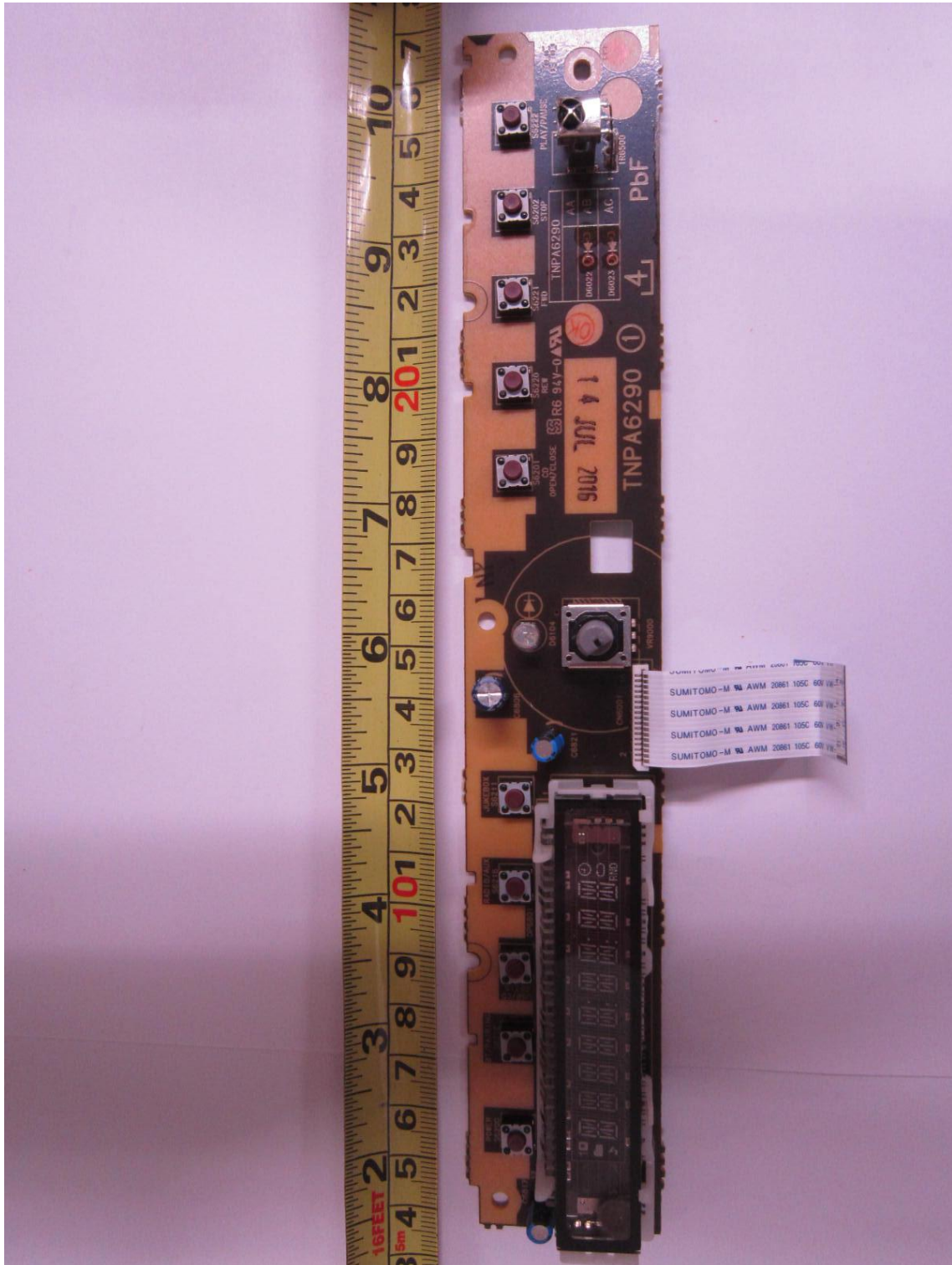
LCD Display Board PCB Component Side
