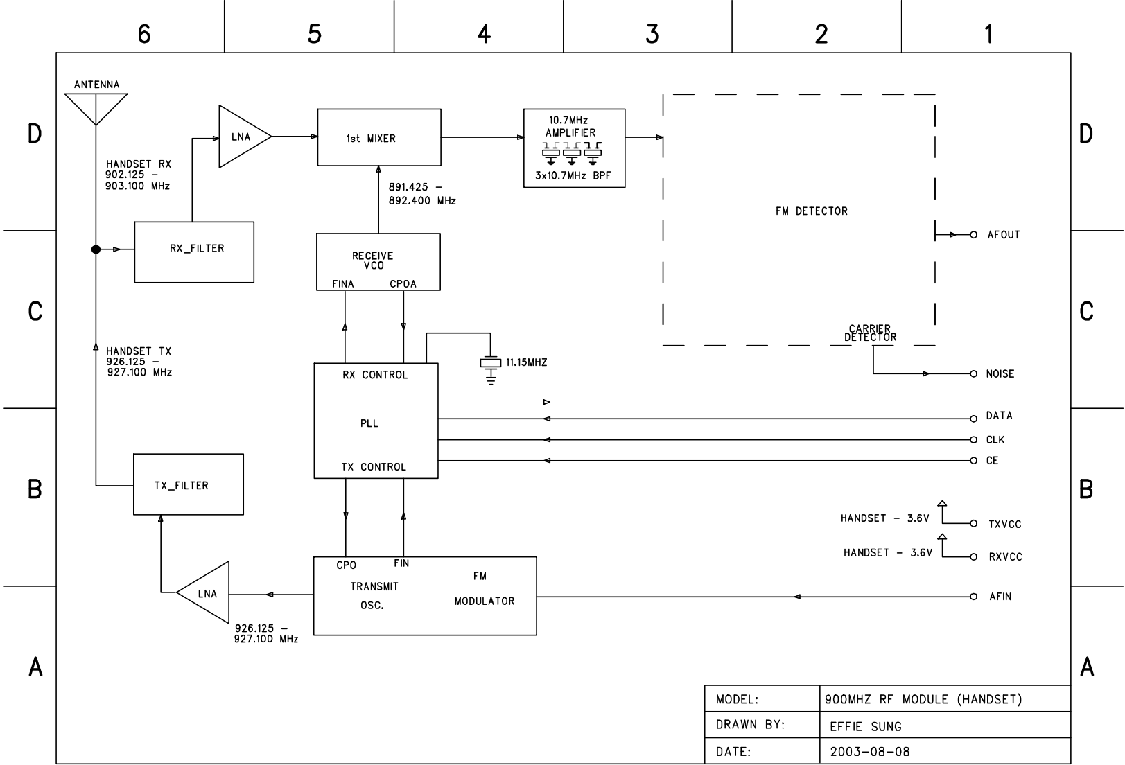
RF Module (Handset) Block Diagram
