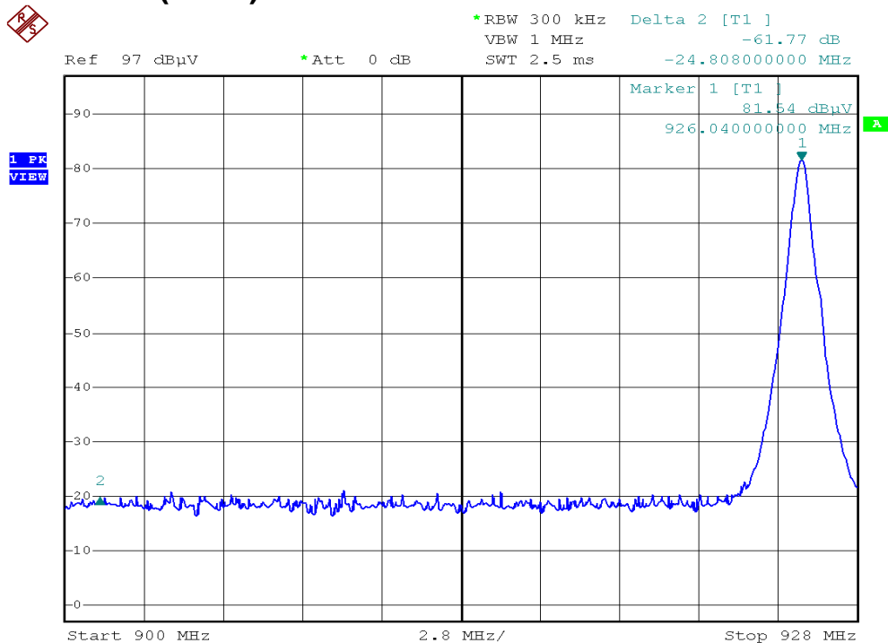
Plot H1A (C410)
