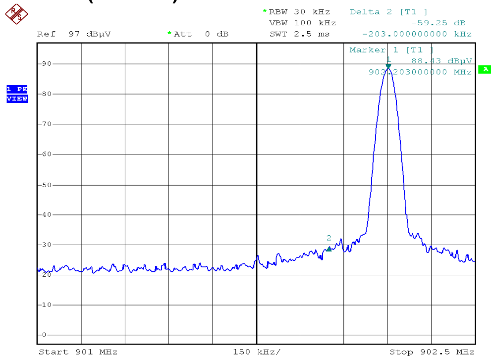
Plot B1A (W425Pro)
