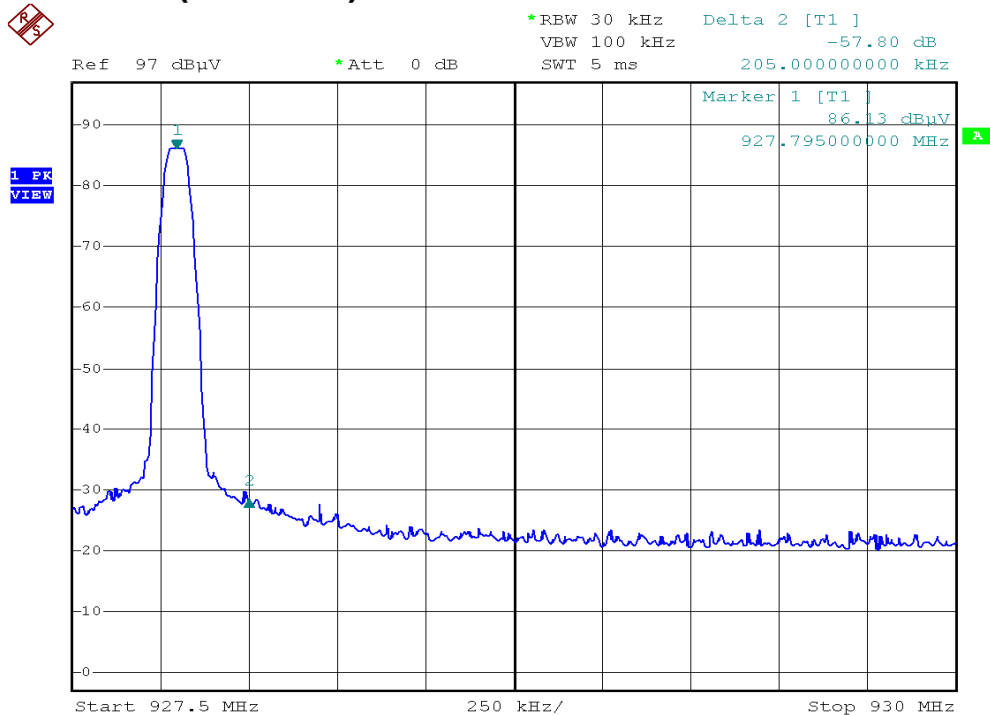
Plot H1B (W425Pro)
