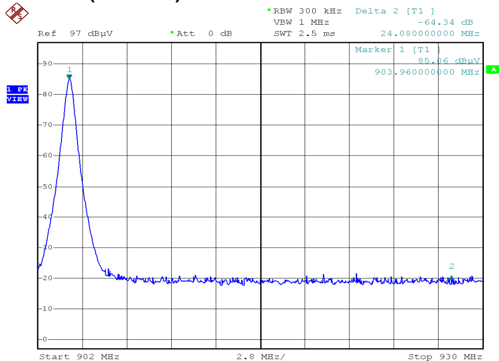
Plot B1B (W425Pro)
