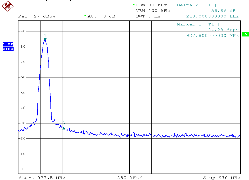
Plot H1B (C410)
