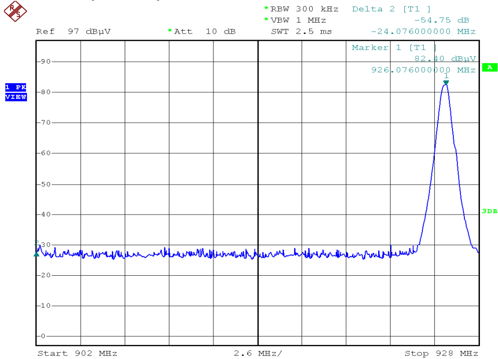
Plot H1A (W425D)
