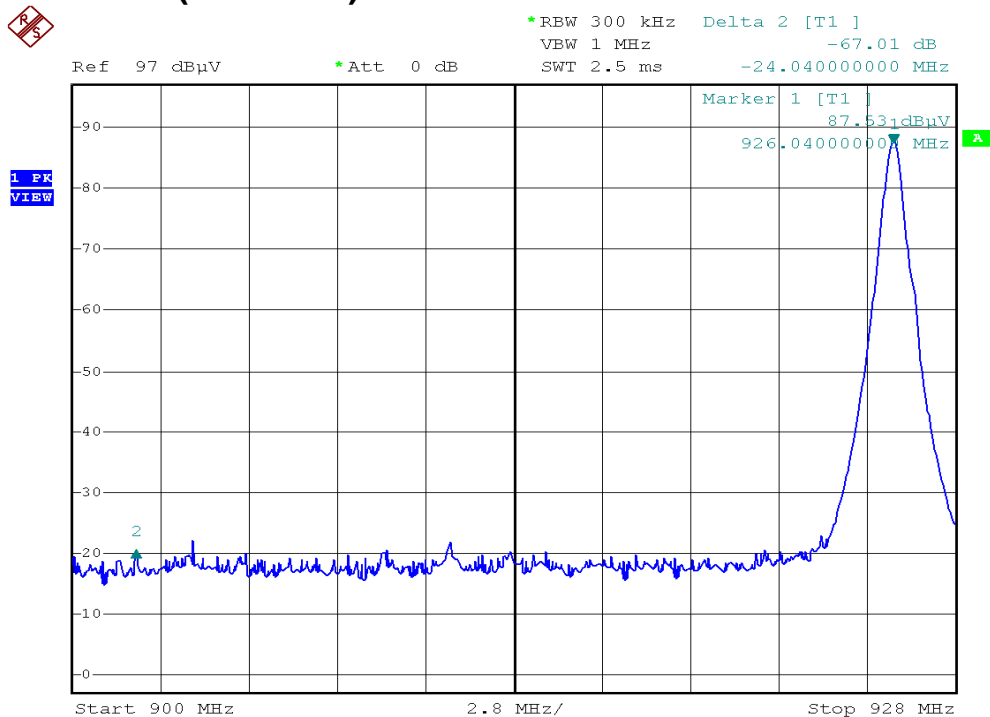
Plot H1A (W425Pro)
