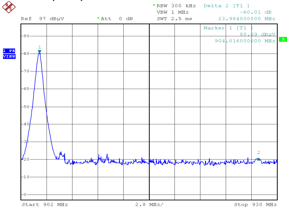
Plot B1B (C410)
