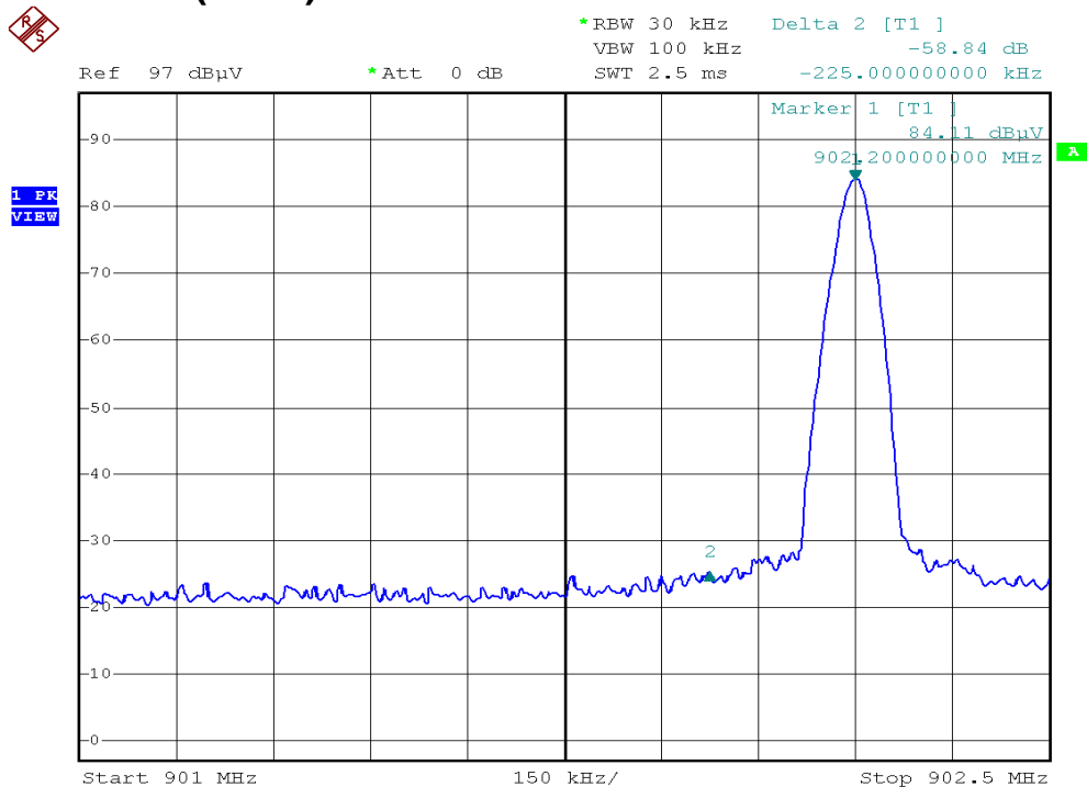
Plot B1A (C410)
