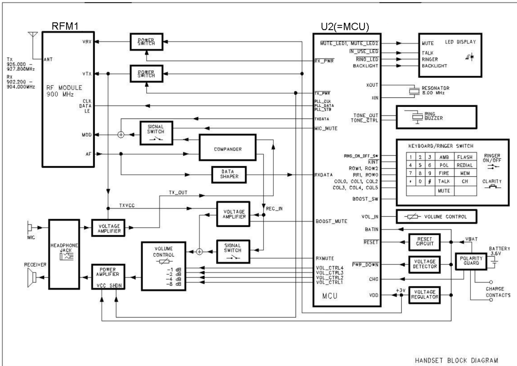
C410 Handset Unit Block Diagram
