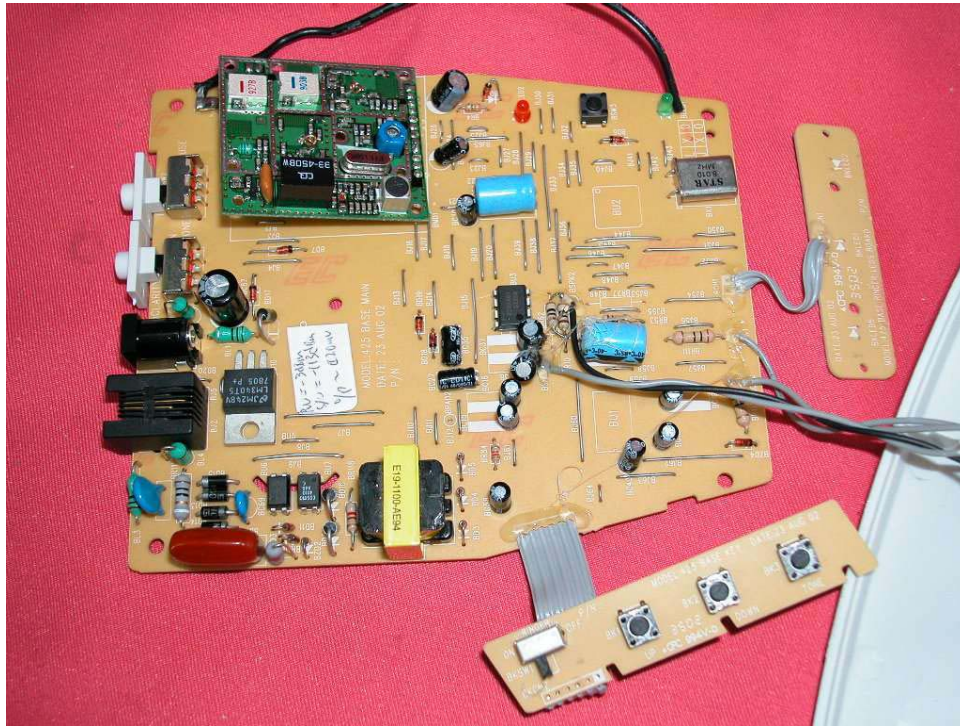
Base Main PCB comp side (view 1)
