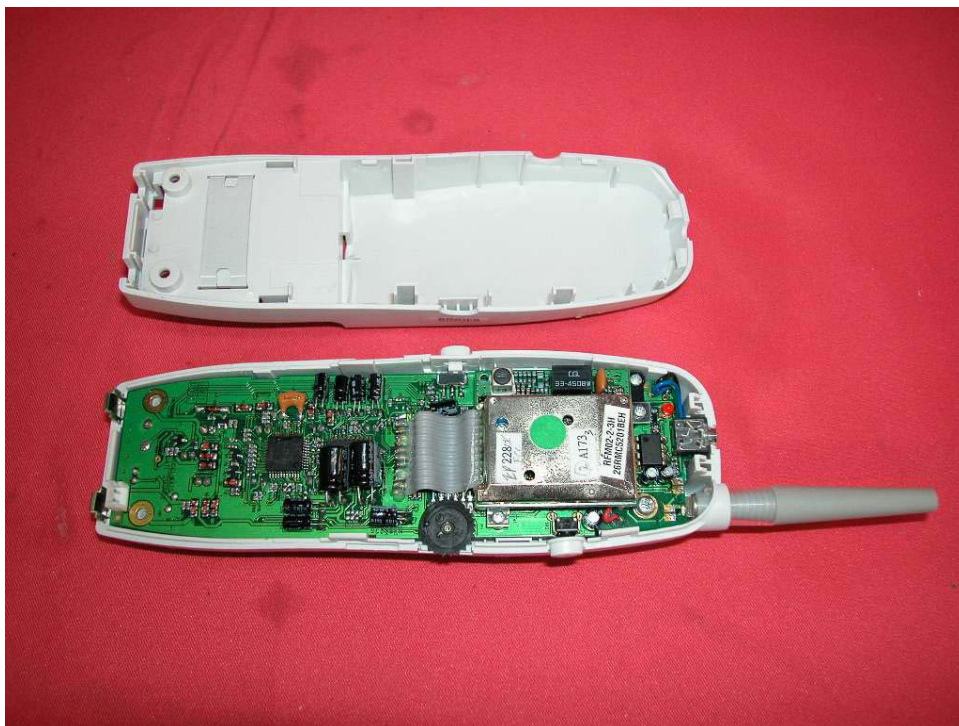
Handset assembly
