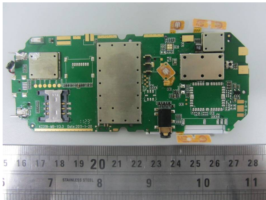
EUT – Main Board Bottom View without GSM Antenna
