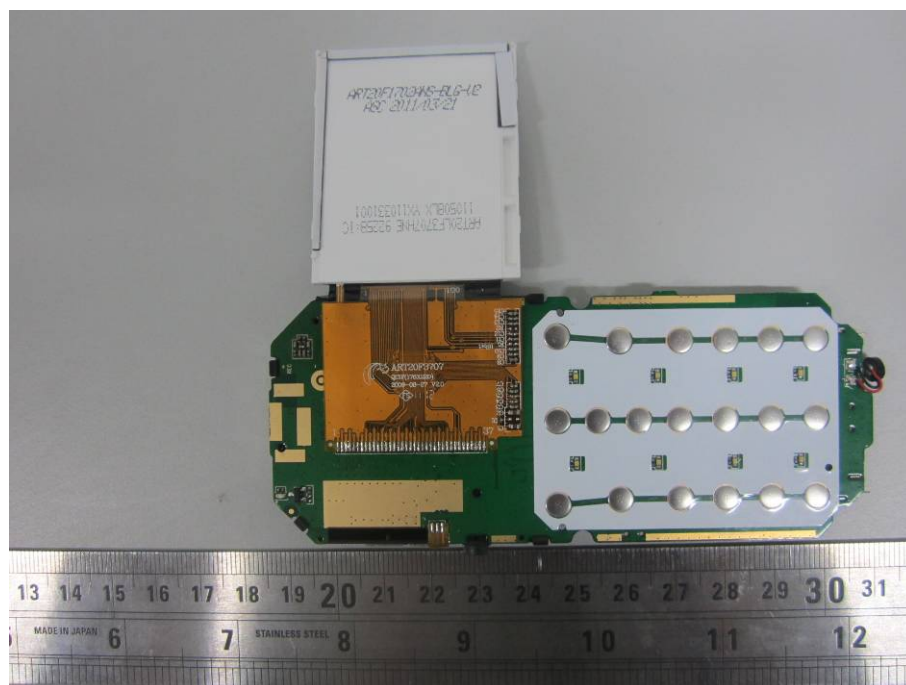
EUT – Main Board Top with LCD Cover off View
