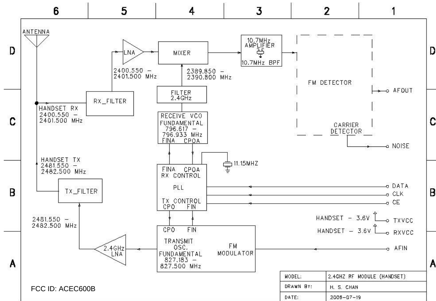
Handset RF Module Block Diagram
