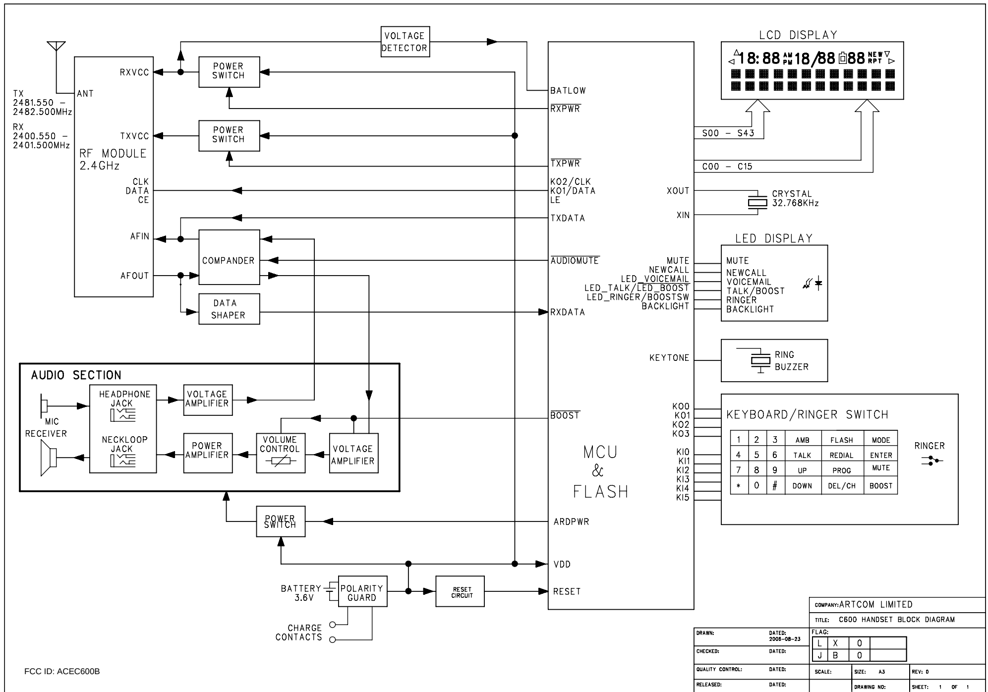
Handset Block Diagram
