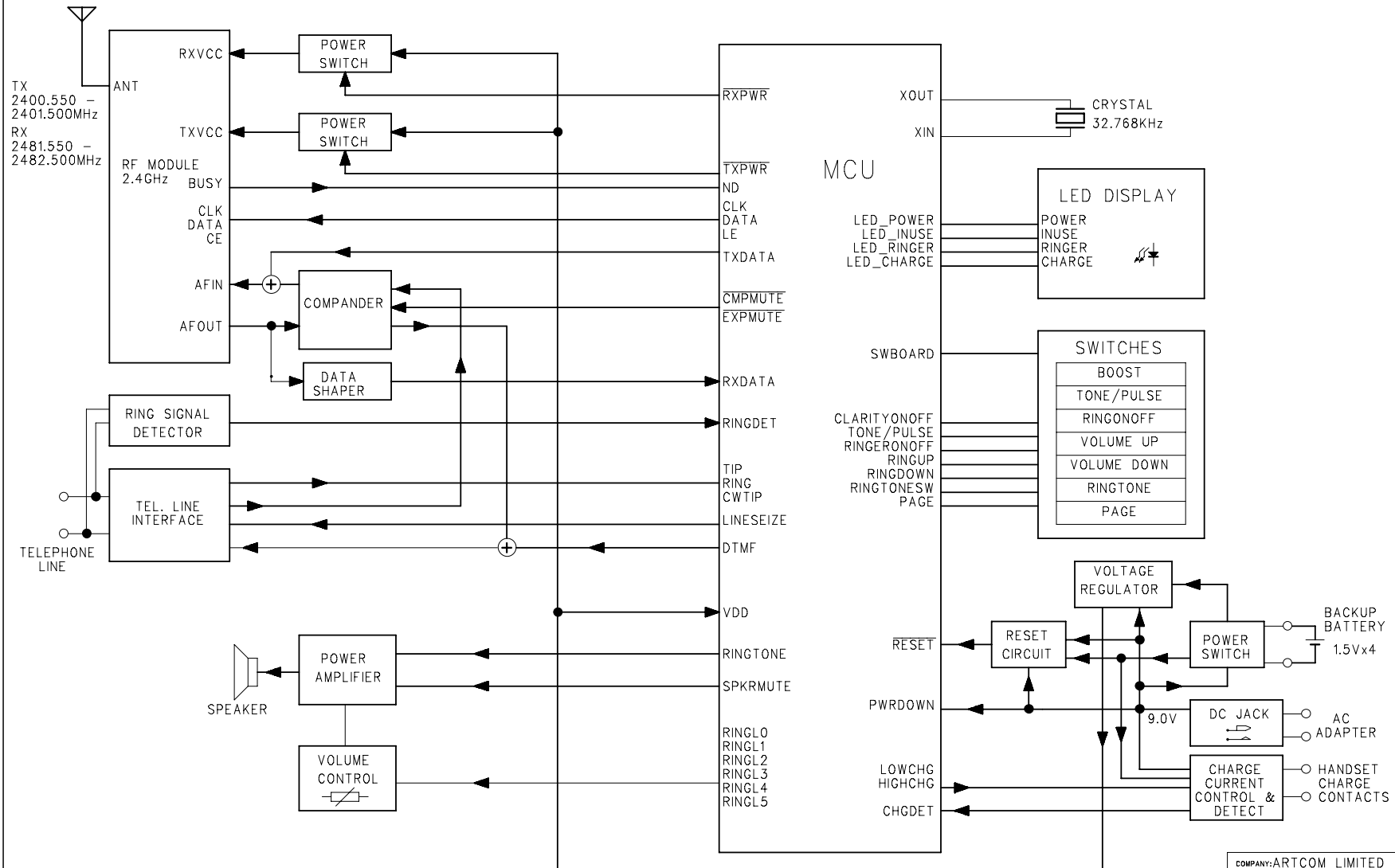
Base Block Diagram
