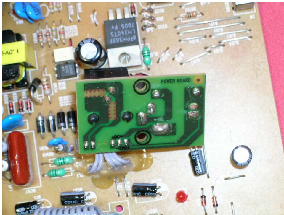
Base Telephone Jack and AC Jack PCB rear side
