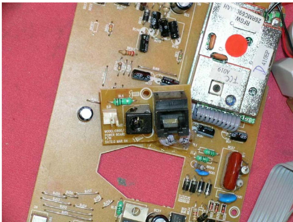
Base Telephone Jack and AC Jack PCB front side
