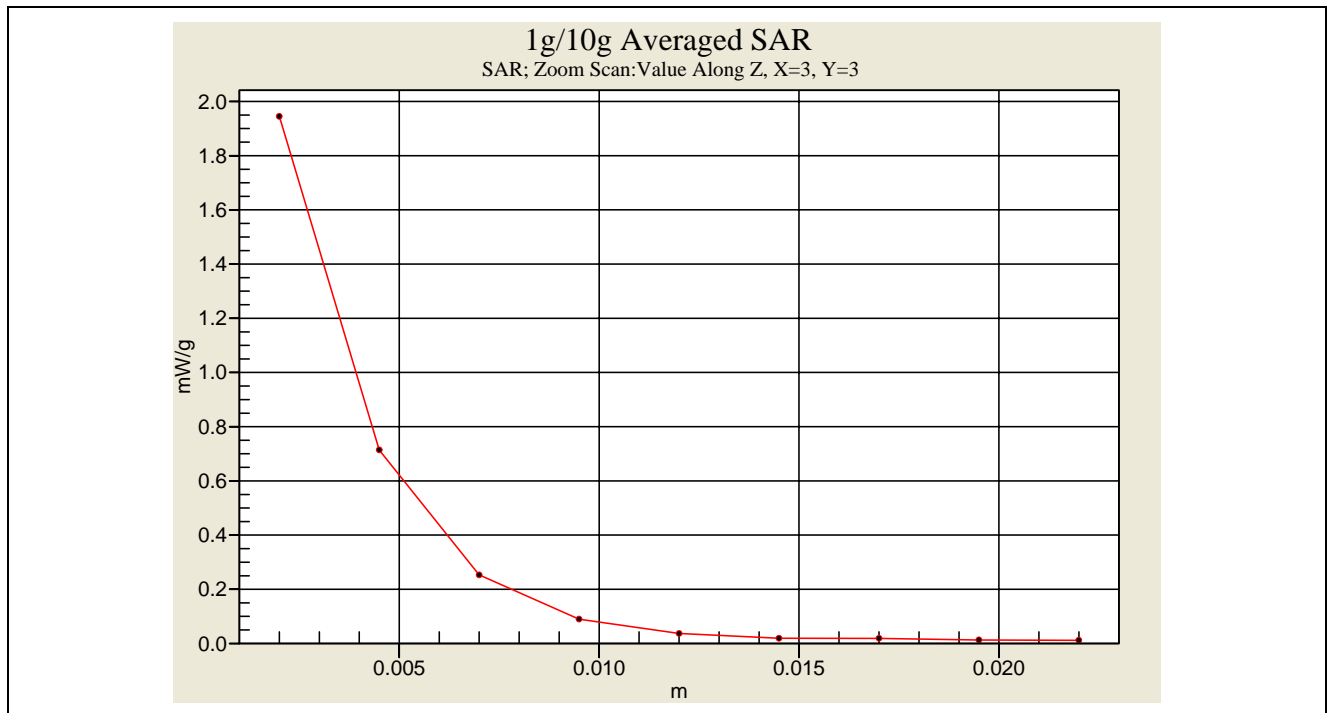
SAR Measurement _ Right Cheek CH81
