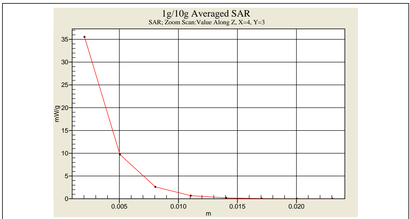
Body-Tissue-Simulating-Liquid 5.8GHz
