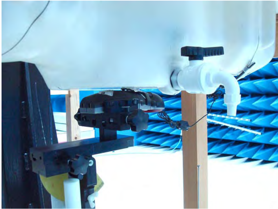
Figure 23. Body SAR Test Setup(Flat Section)_ Headset
