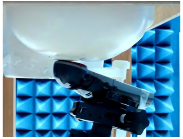
Figure 18. Right Head SAR Test Setup (Tilted)
