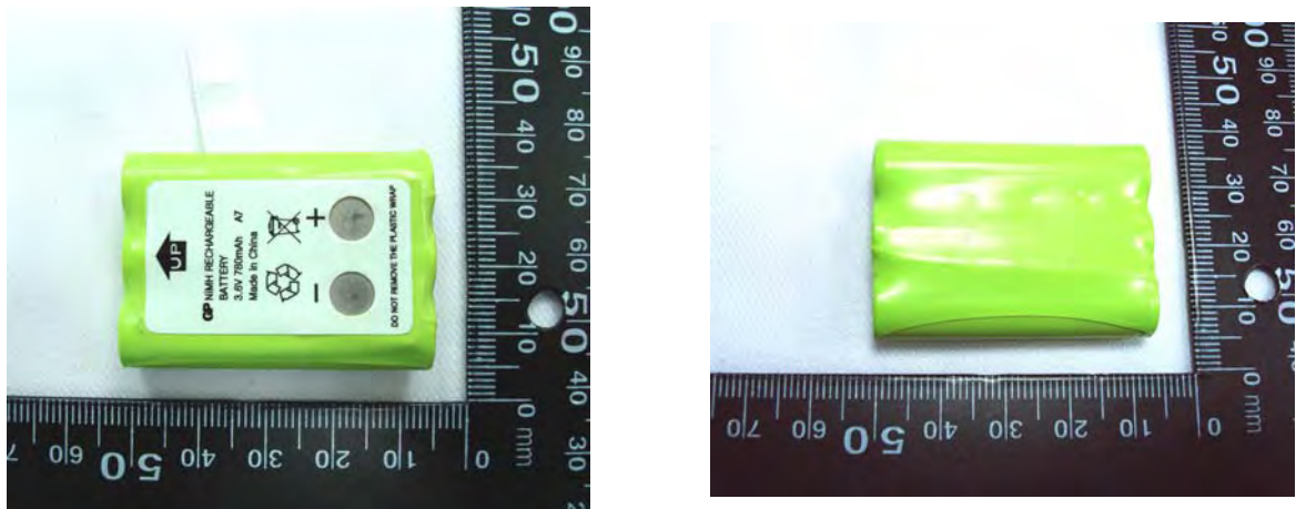
Figure 5. Battery (Ni-MH 3.6V , 780mAh)
