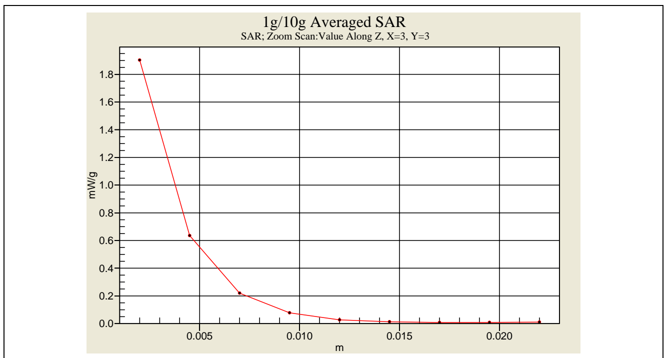
SAR Measurement _ Flat 15mm space CH81
