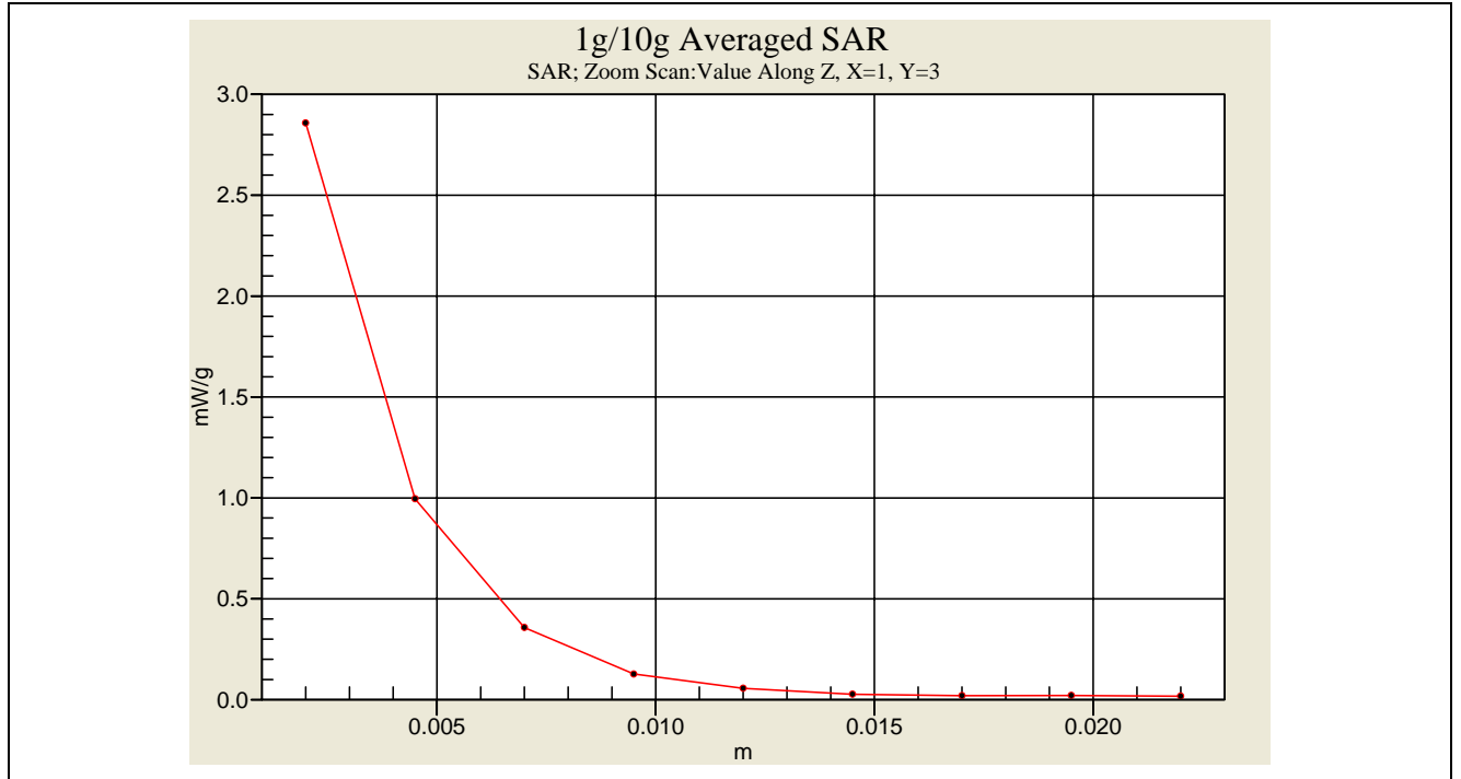
SAR Measurement _ Flat attach belt clip with Neck Loop CH81
