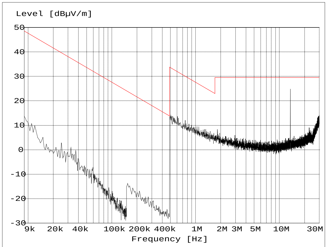
Figure B – 3 Radiated Spurious Emissions, 9 kHz to 30 MHz, 65 x 40 mm Loop Antenna
