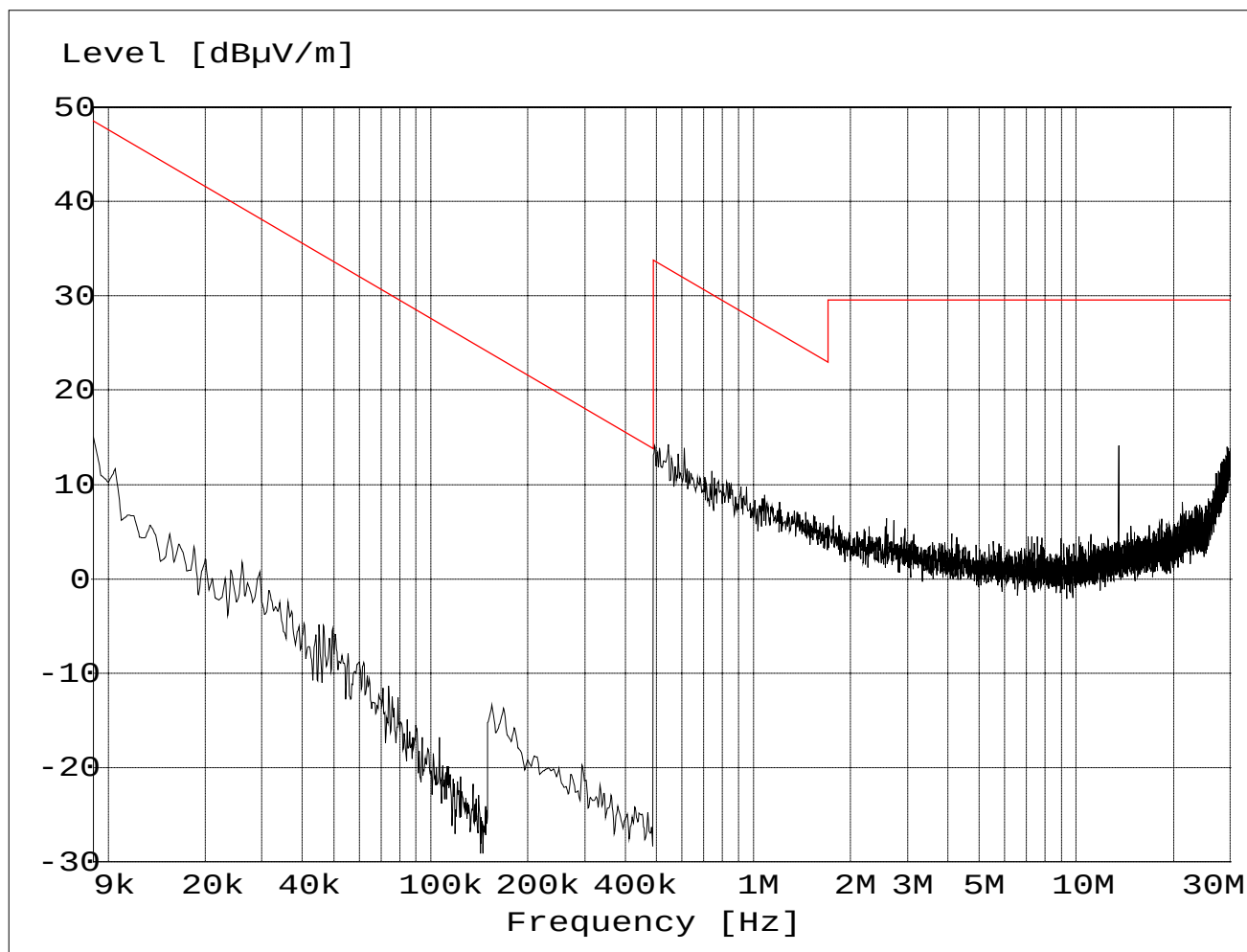
Figure B – 4 Radiated Spurious Emissions, 9 kHz to 30 MHz, 50 x 25 mm w/ferrite Loop Antenna
