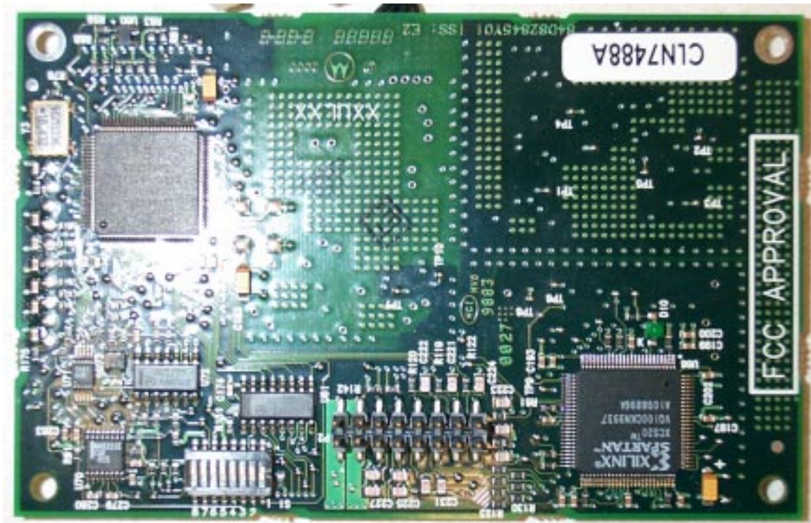
Figure 3.0-2 Control PCB back view
