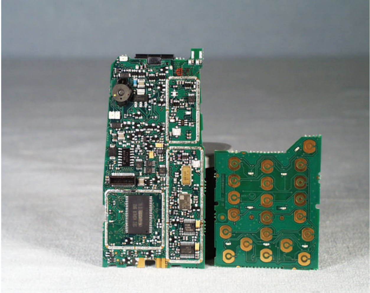
Solder side of the interface board (Without RF Cans)
