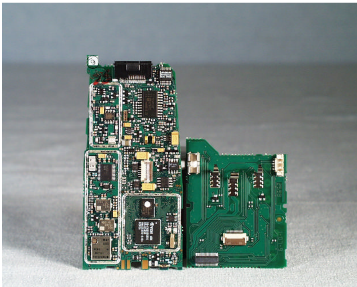
Component side of the interface board (Without RF Cans)
