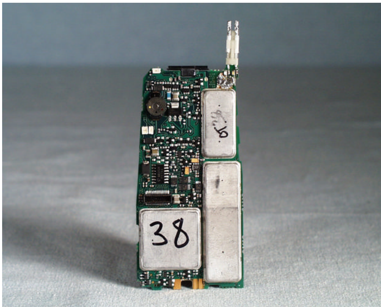
Solder side of the interface board (With RF Cans)
