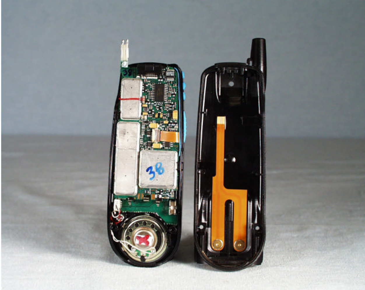
Inside View of the AAS19ZAN9121AA
