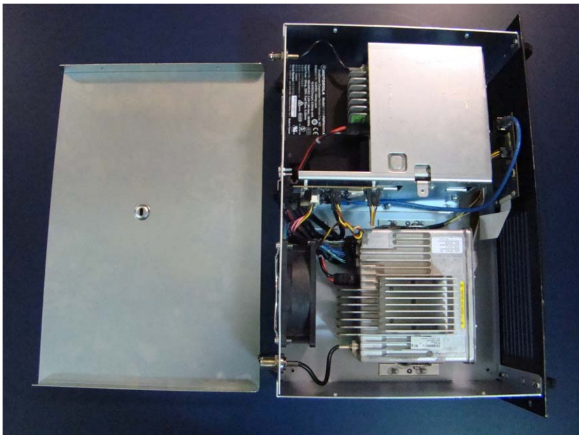
TOP VIEW OF WITH TOP COVER REMOVED
