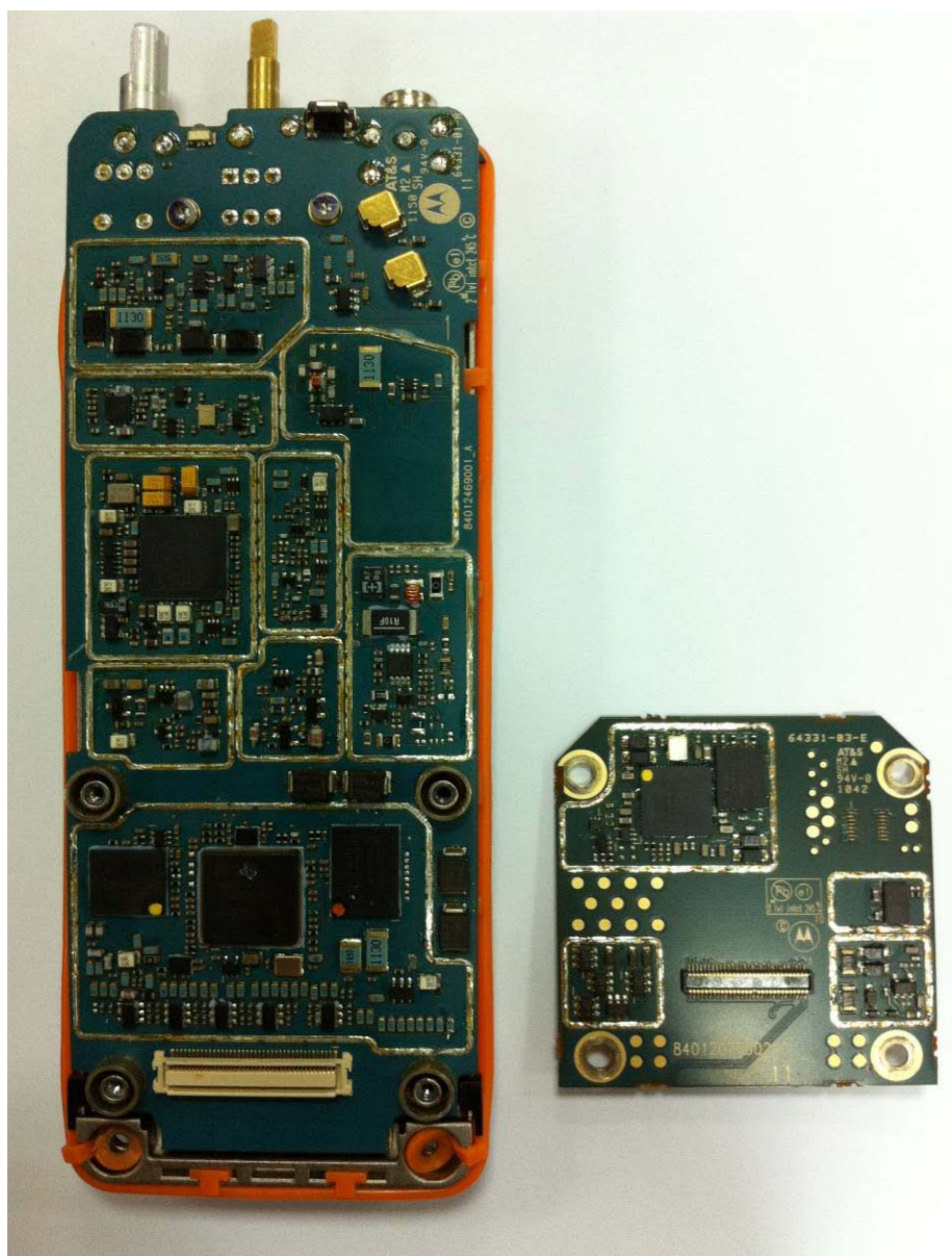
FIGURE 3- 3: NEO CSA WITH OPTION BOARD WITHOUT SHIELDS (TOP SIDE)
