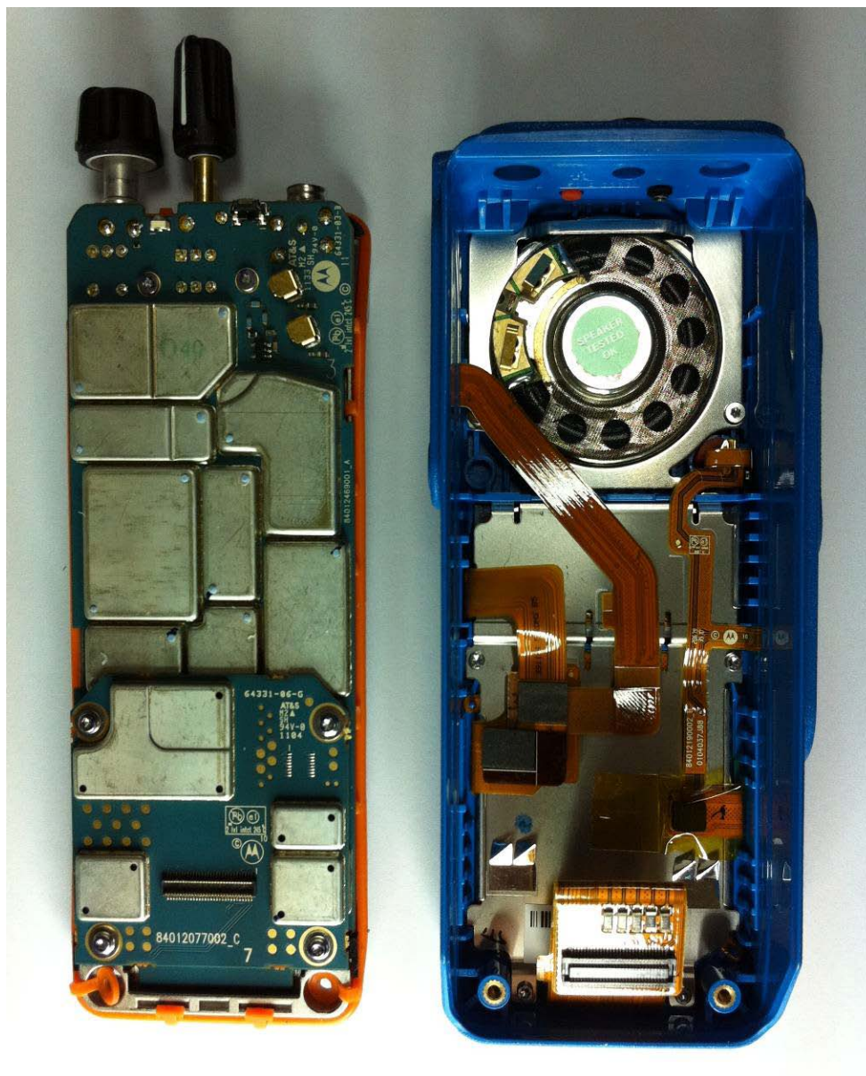
FIGURE 3- 1: NEO CSA COMPLETE INTERNAL OPEN UP VIEW.
