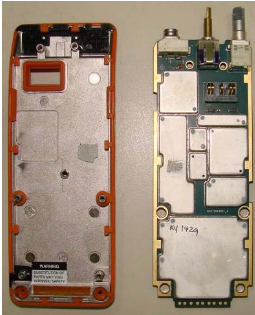
FIGURE 3-5: NEO CSA CHASSIS, BOARD AND CAN SHIELDS
