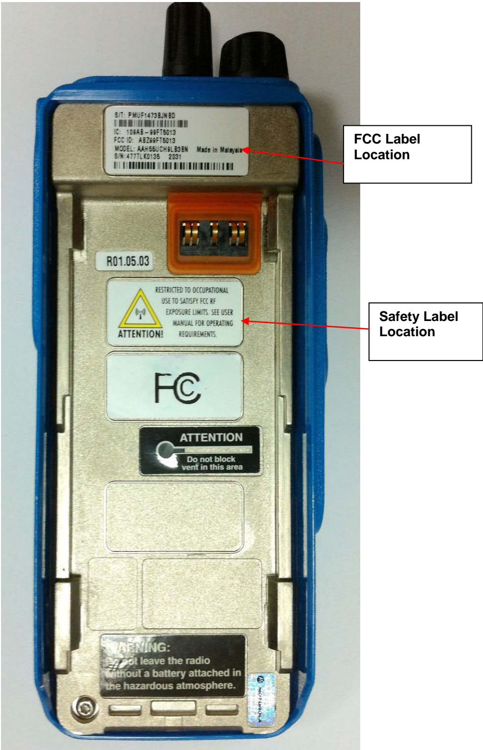
FIGURE 3-5: FCC AND SAFETY LABELS LOCATION OF PORTABLE RADIO
