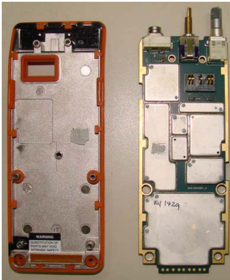
FIGURE 3-3: NEO CSA CHASIS, BOARD AND CAN SHIELDS
