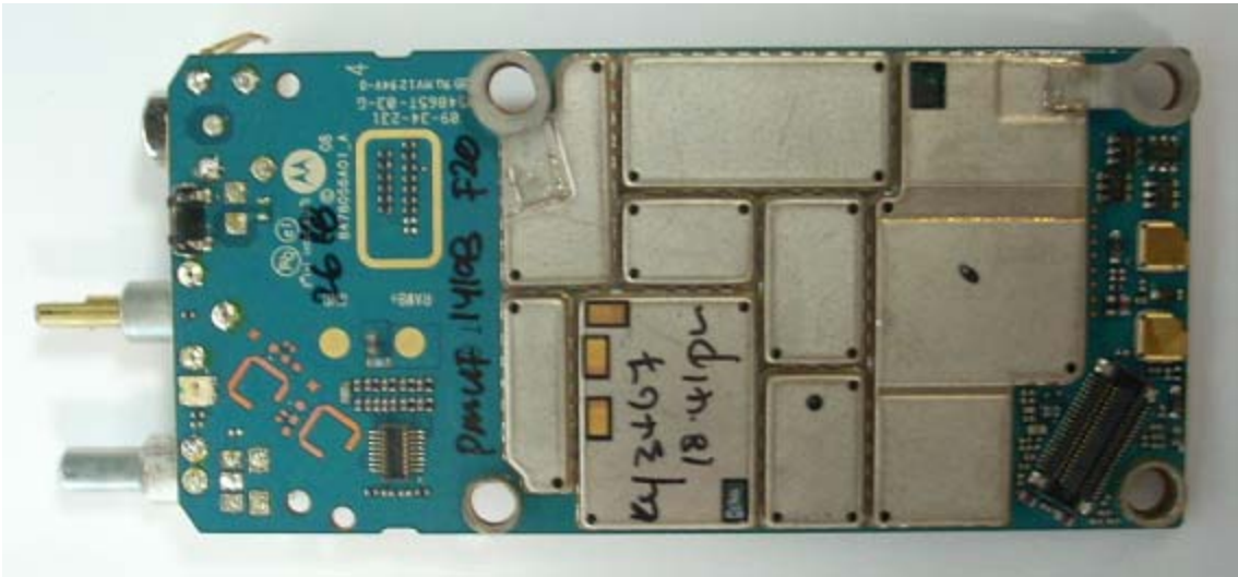
FIGURE 3-7: MOTOTRBO BOARD TOP VIEW.
