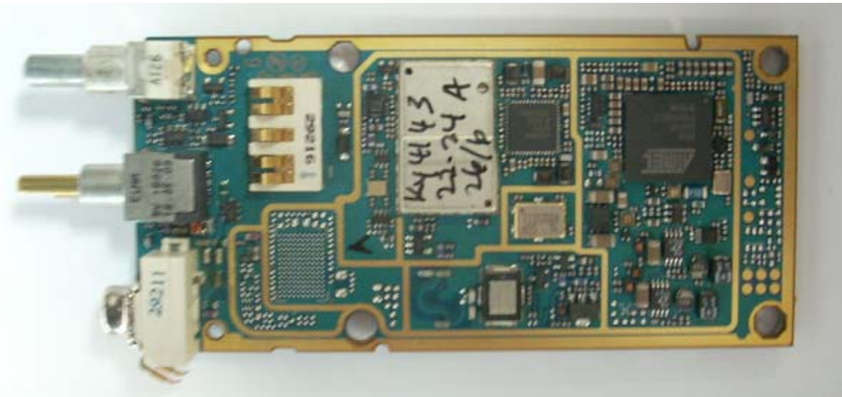
FIGURE 3-5: MOTOTRBO BOTTOM VIEW BOARD WITHOUT GPS.
