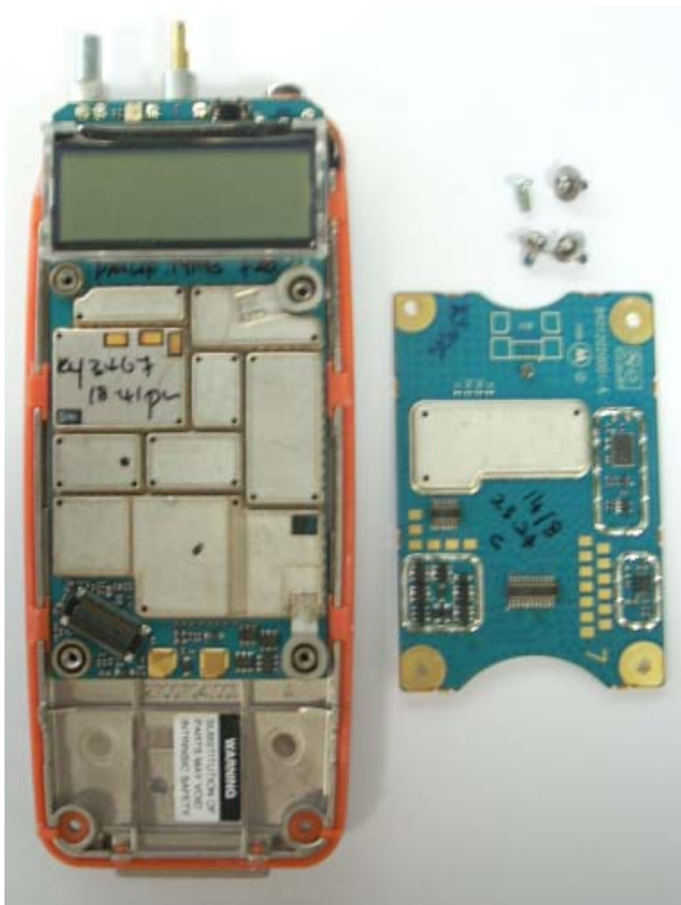
FIGURE 3- 2: MOTOTRBO WITH OPTION BOARD.
