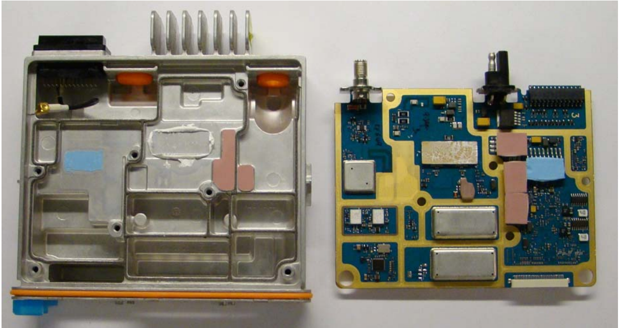
TOP VIEW OF GPS MODEL WITH CIRCUIT BOARD REMOVED FROM CHASSIS (MATING SURFACES OF CIRCUIT BOARD AND CHASSIS ARE SHOWN)
