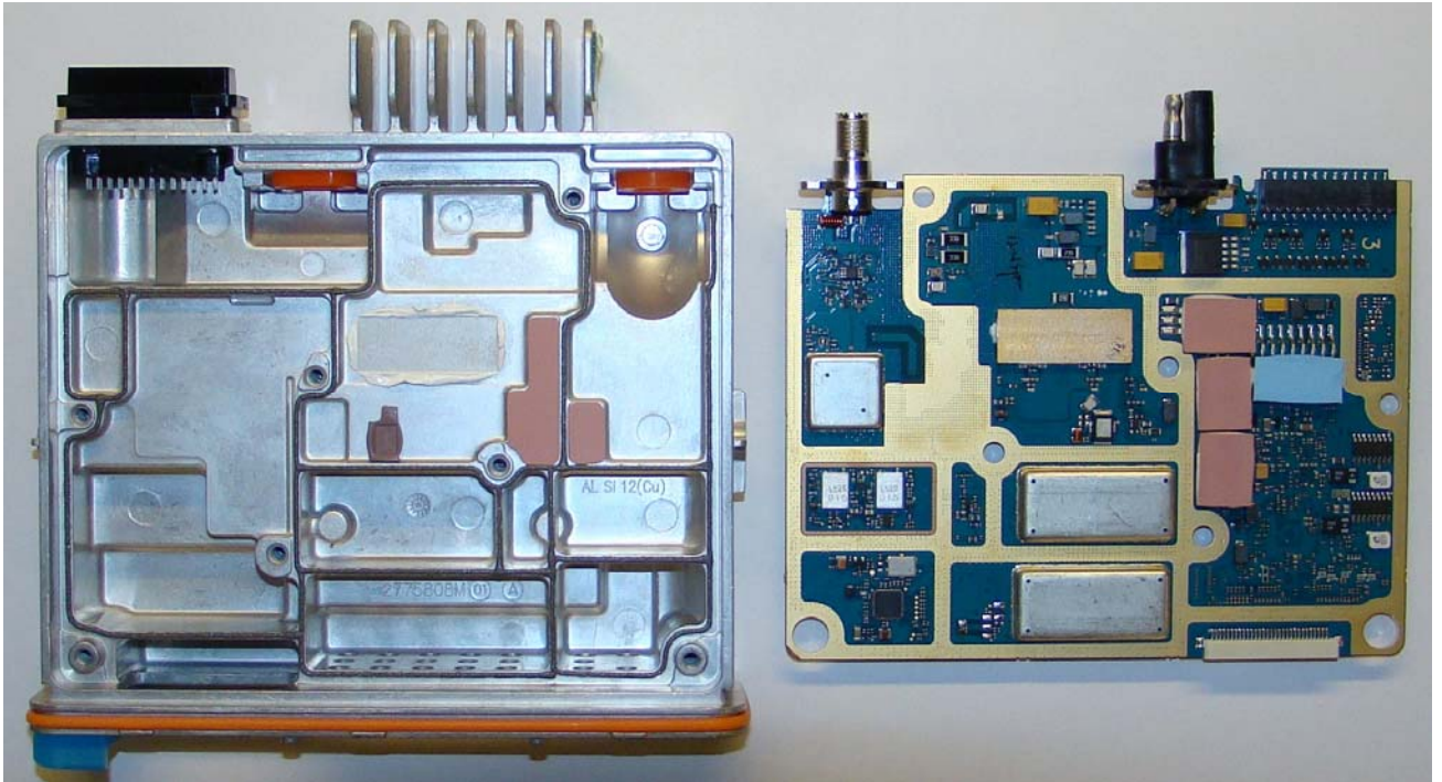
TOP VIEW OF NON-GPS MODEL WITH CIRCUIT BOARD REMOVED FROM CHASSIS (MATING SURFACES OF CIRCUIT BOARD AND CHASSIS ARE SHOWN)
