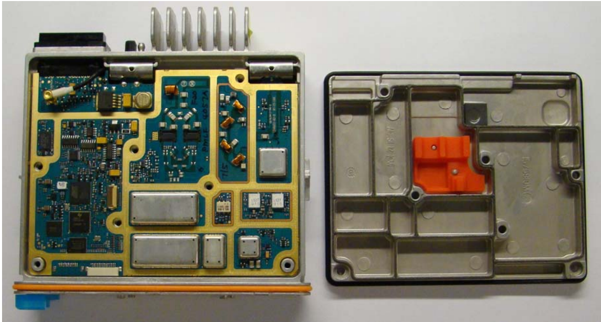
TOP VIEW OF GPS MODEL WITH CHASSIS TOP COVER REMOVED (MATING SURFACES OF TOP COVER AND CIRCUIT BOARD IN CHASSIS ARE SHOWN)
