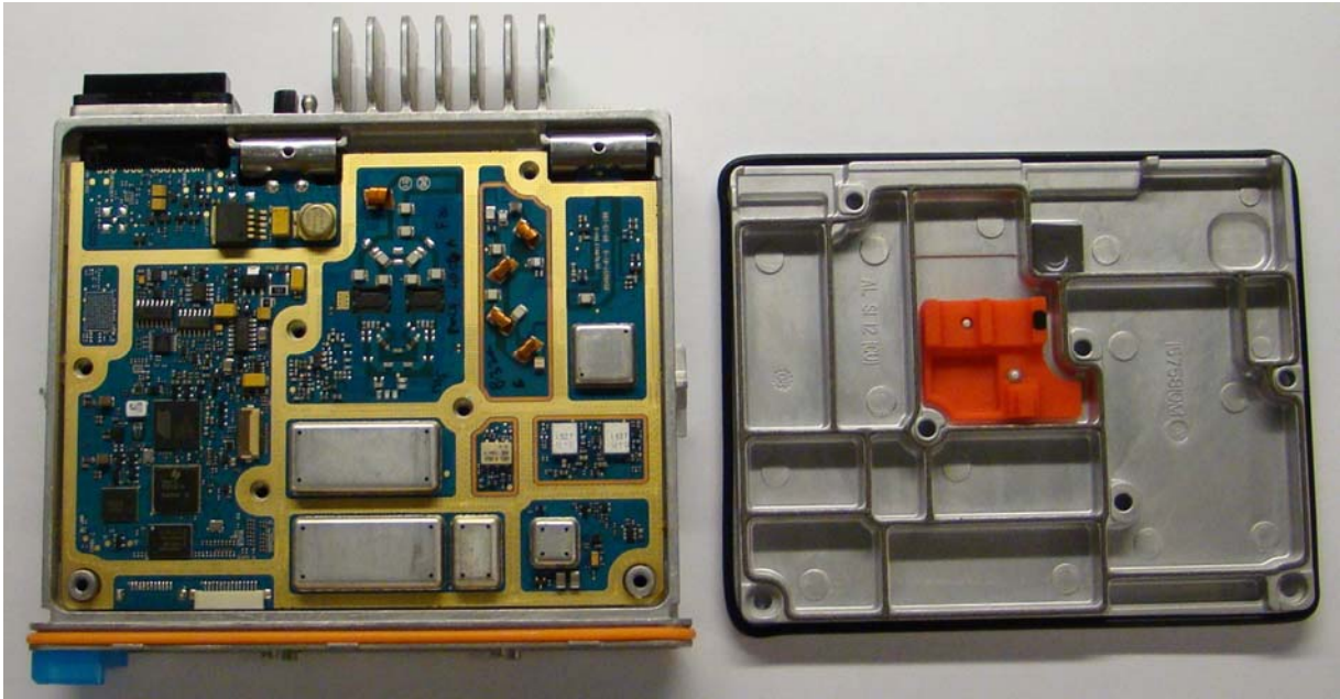
TOP VIEW OF NON-GPS MODEL WITH CHASSIS TOP COVER REMOVED (MATING SURFACES OF TOP COVER AND CIRCUIT BOARD IN CHASSIS ARE SHOWN)
