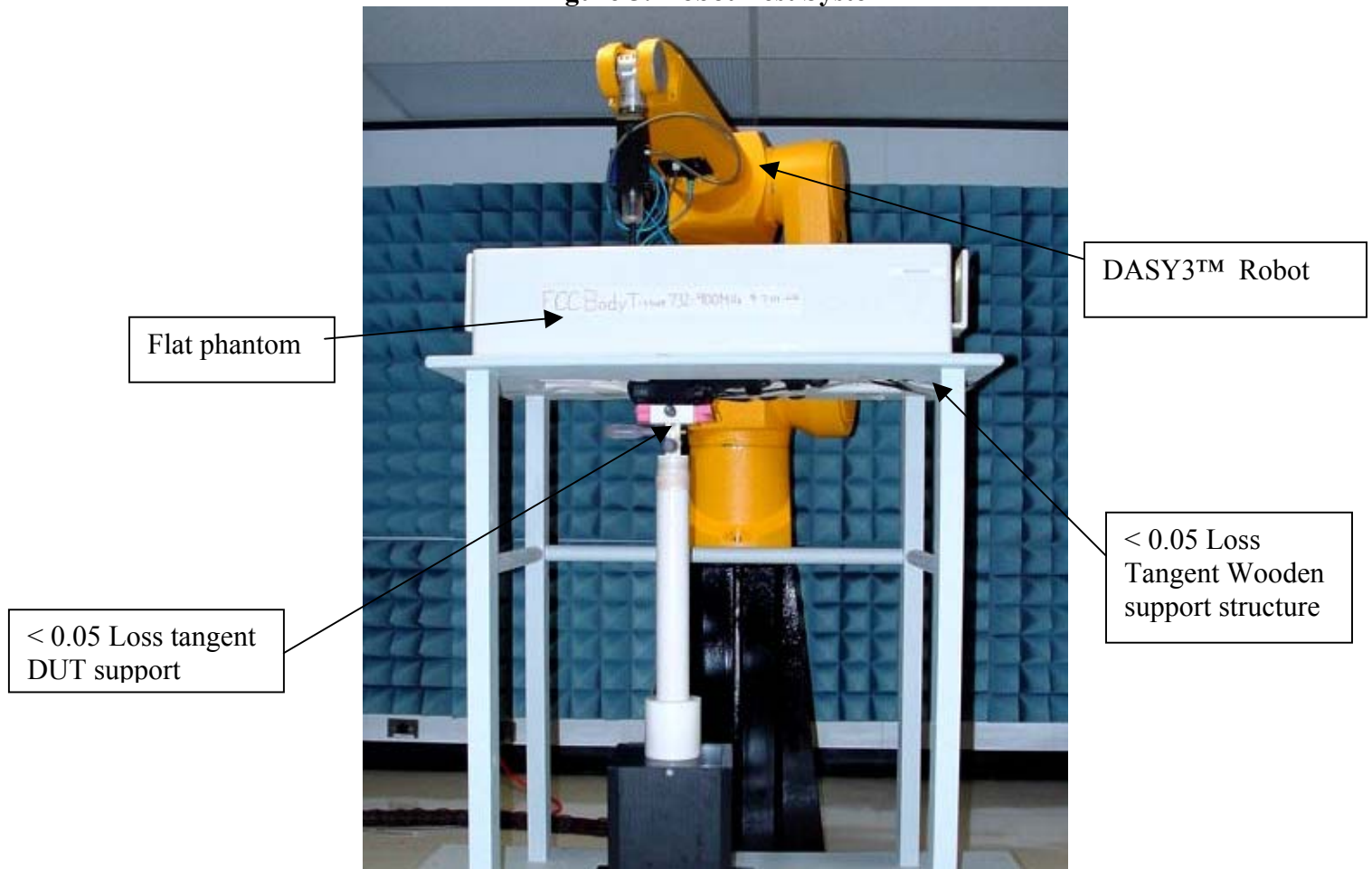
Figure 5: Robot Test System
