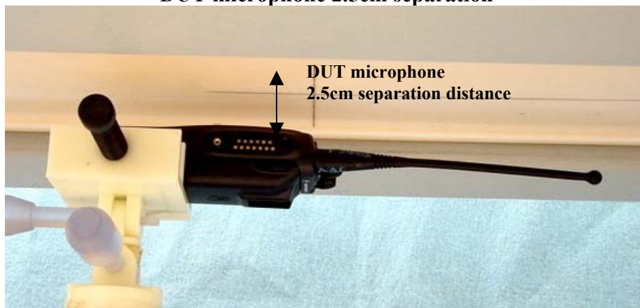
Figure 4: Assessment at the Face; DUT microphone 2.5cm separation
