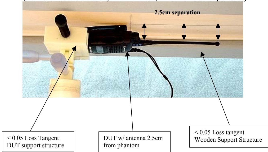
Figure 1: Highest S.A.R. configuration. Assessment at the Abdomen; (DUT with audio accessory PMLN4418A; Antenna 2.5cm separation)
