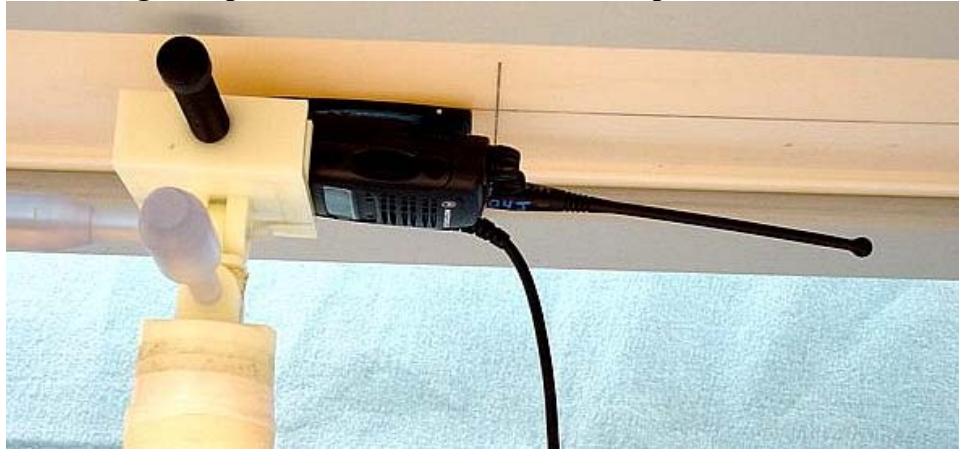
Figure 2: Assessment at the Abdomen; DUT Against phantom w/ HLN9714A belt clip and attached RSM
