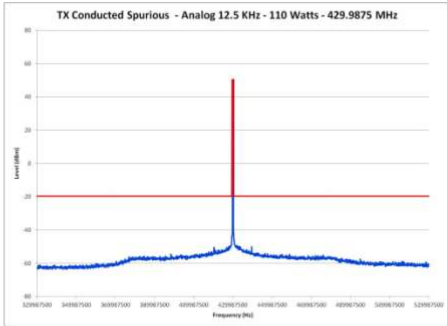
E1-6.5 Conducted Spurious Emission Spectrum, 200 MHz Span, Power 110 Watts, 429.9875 MHz
