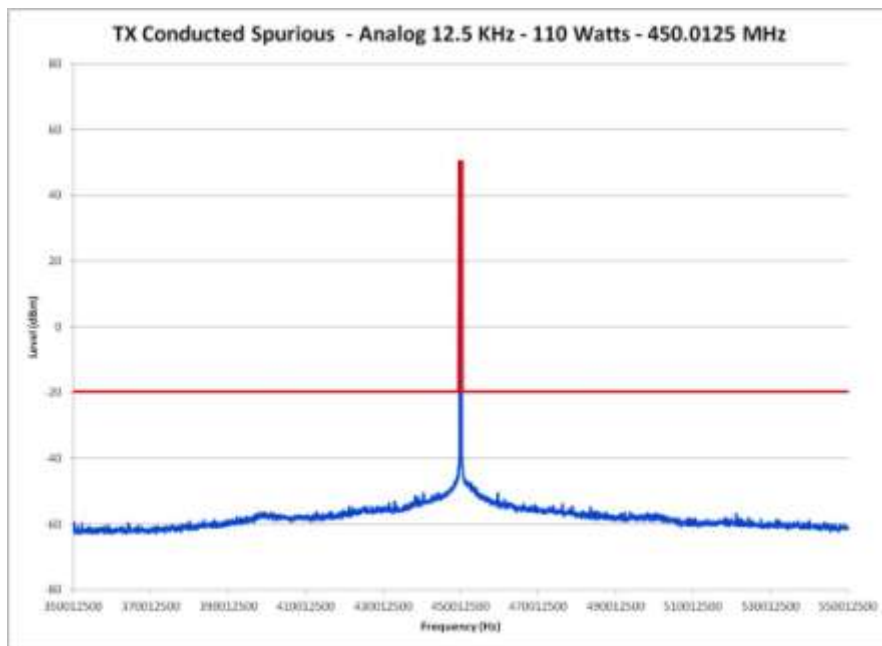
E1-6.6 Conducted Spurious Emission Spectrum, 200 MHz Span, Power 110 Watts, 450.0125 MHz
