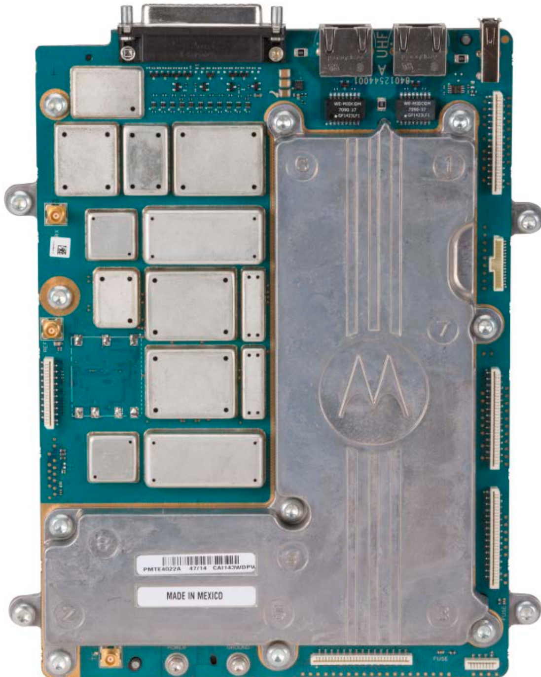
Internal Front View – Modem Module
