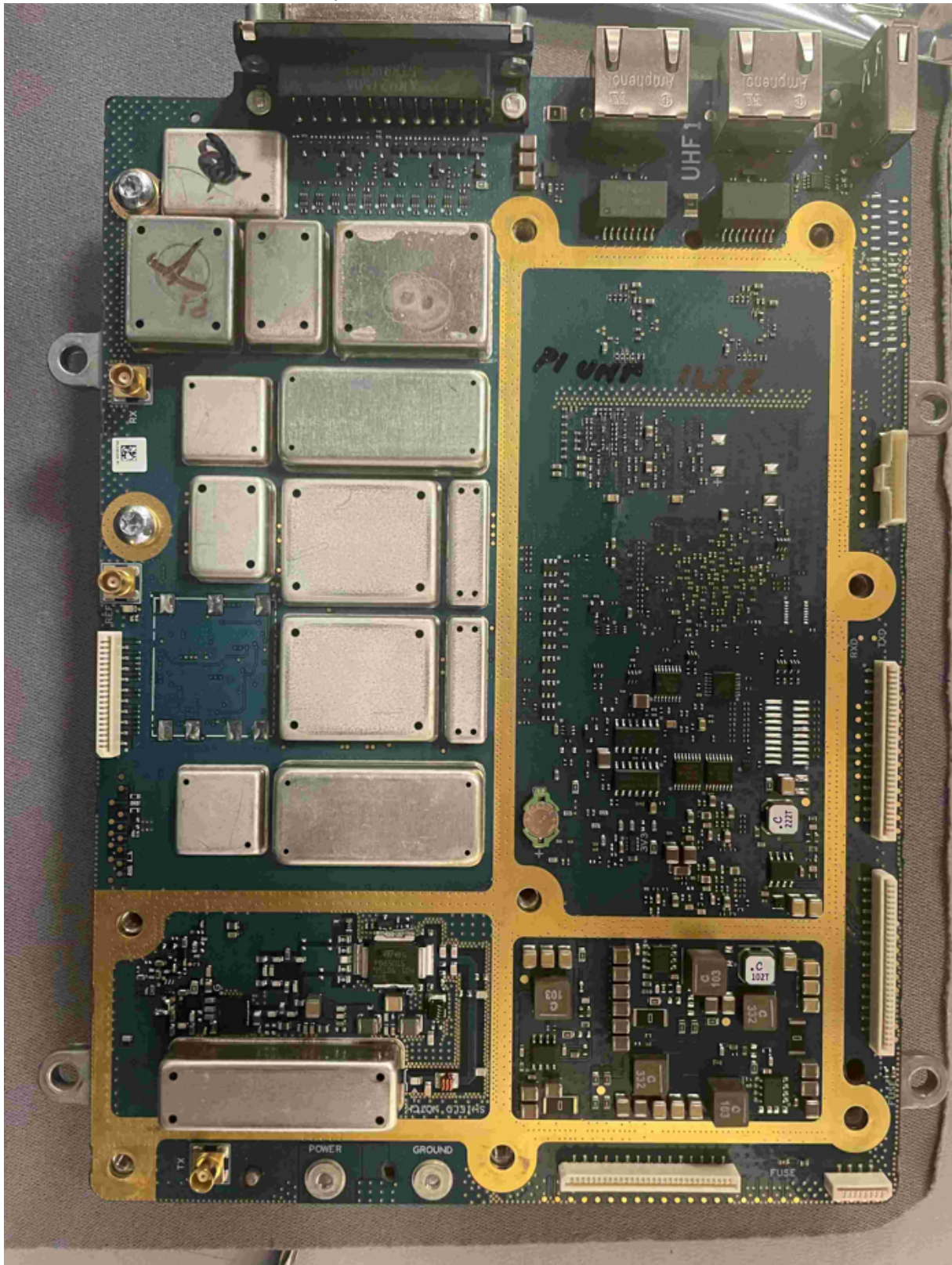
Internal Front View – Modem Module Top View – Cover Removed
