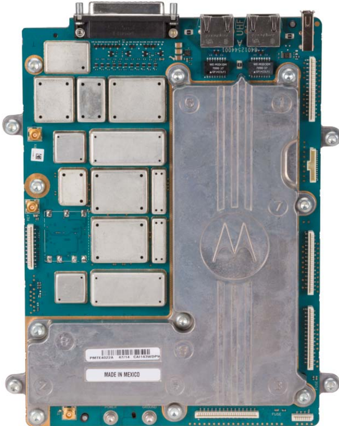
Internal Front View – Modem Module
