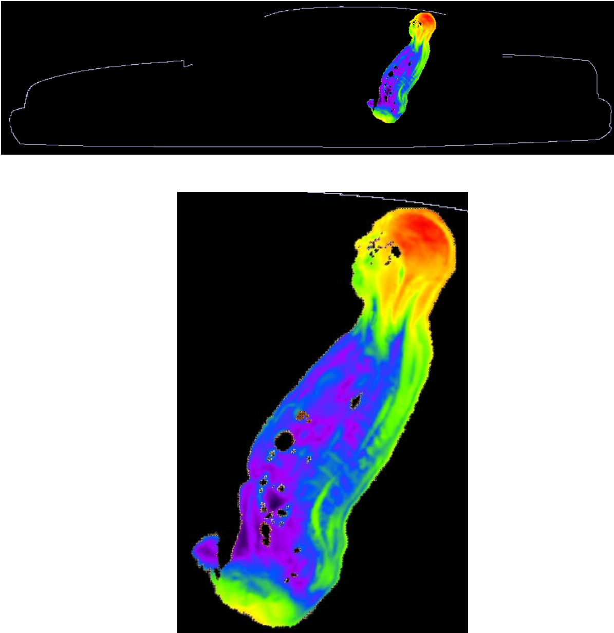
Figure 3. SAR distribution at 406.125 MHz in the passenger model located on the side of the back seat, produced by the trunk-mount HAE6022A antenna. The contour plot is relative to the plane where the peak 1-g average SAR for this exposure condition occurs.
