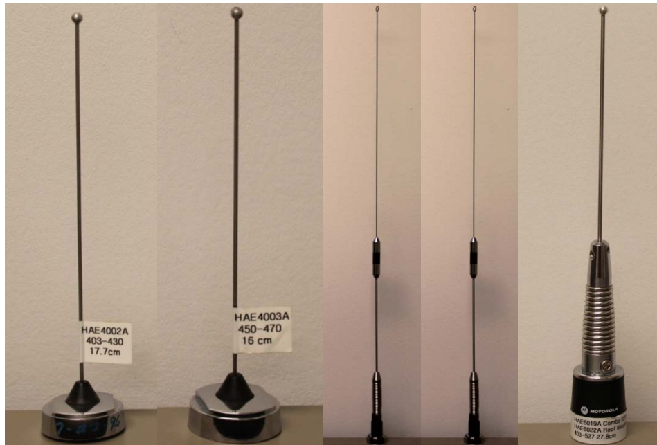
UHF Antenna kit numbers, from left to right: HAE4002A, HAE4003A, HAE4010A, HAE4011A, and HAE6022A (pictures not to scale)
