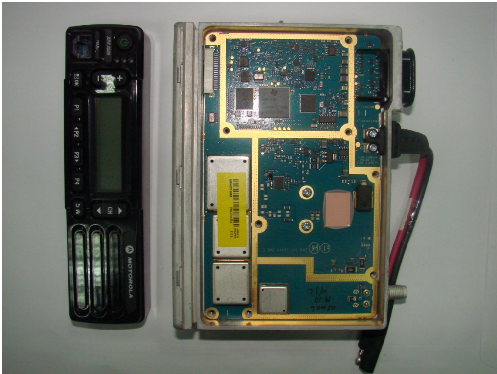
RF board with chassis and control head (Top)
