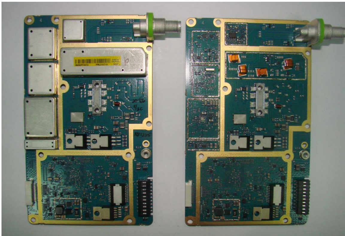
RF board with and without shields (Top)
