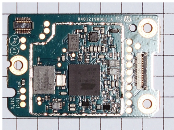
GOB board without shield (Bottom)
