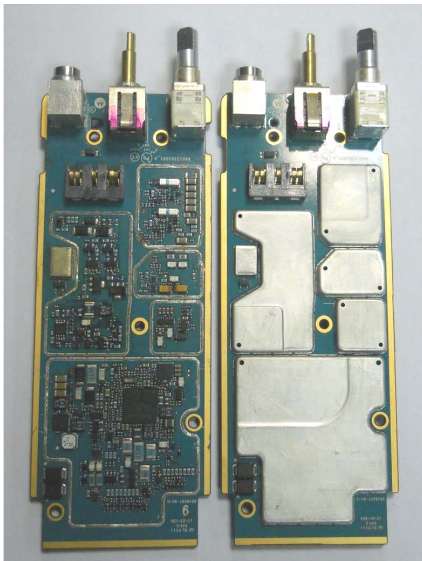
RF board without & with Shields (Bottom)
