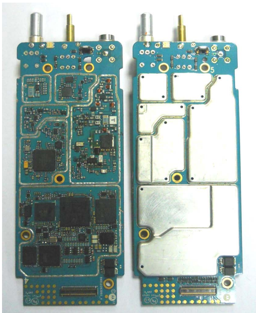
RF board without & with Shields (Top)
